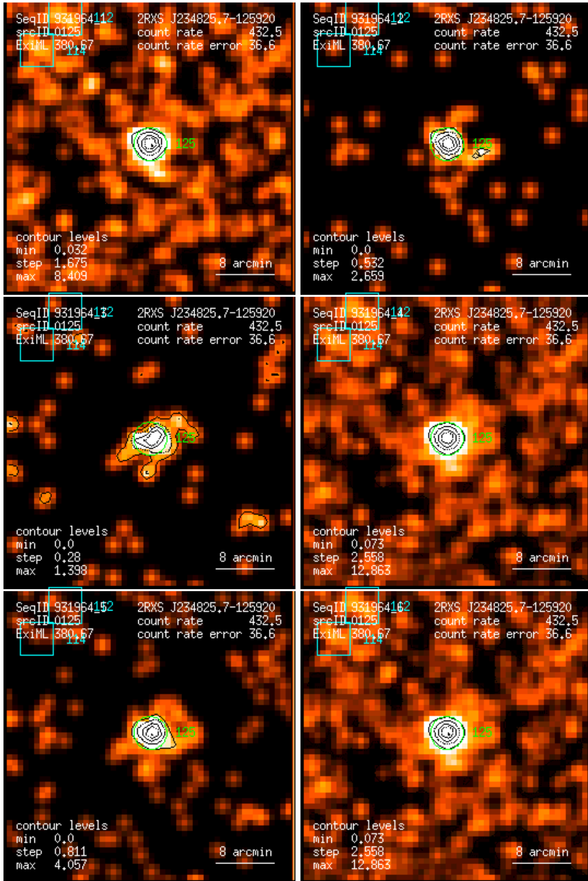
Figure 125: RASS 931964: detection 0125: band rate images, Gaussian filter: (1) PSPC channels 11 – 41, (2) 52 – 90, (3) 91 – 201, (4) 11 – 235, (5) 52 – 201, (6) 11 – 201. Broad band rates in counts/ks. Band rate contour levels in counts/ks/arcmin 2 .
