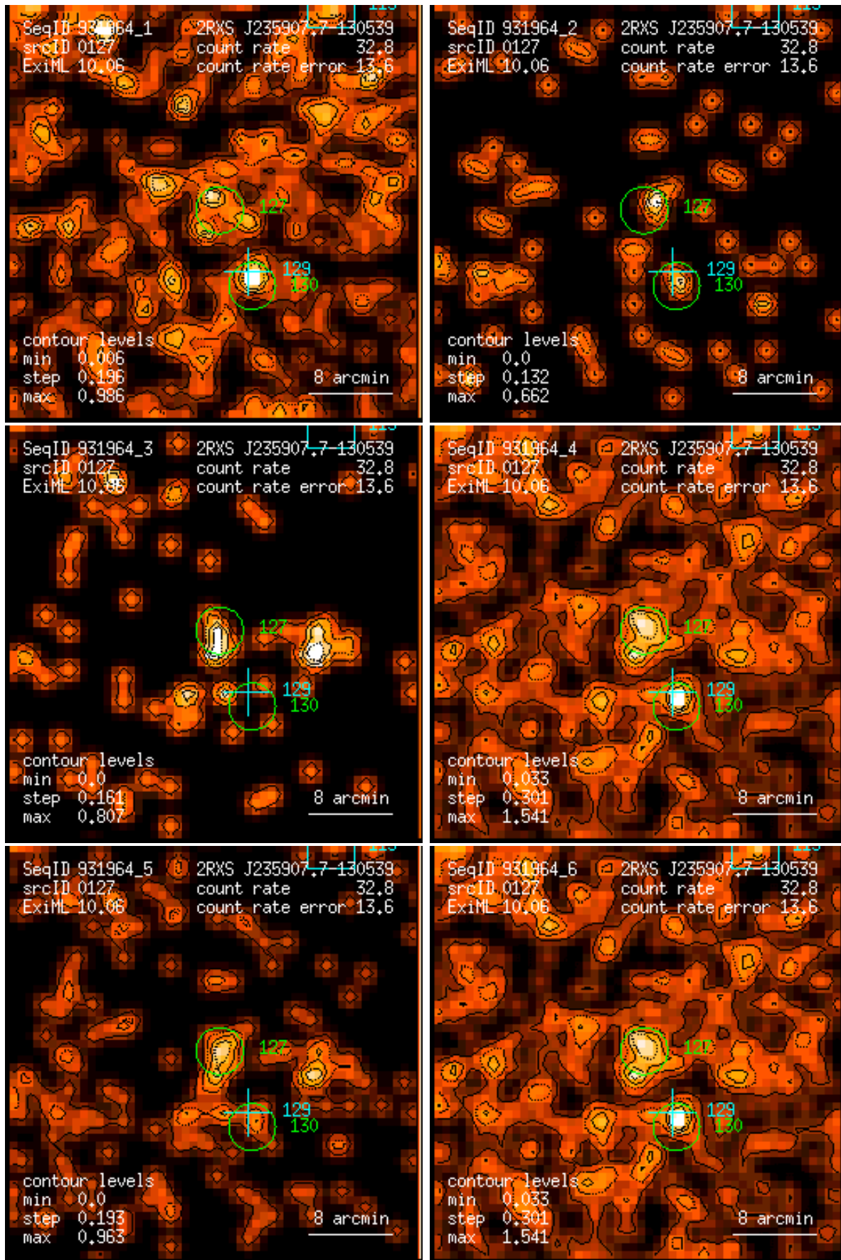
Figure 127: RASS 931964: detection 0127: band rate images, Gaussian filter: (1) PSPC channels 11 – 41, (2) 52 – 90, (3) 91 – 201, (4) 11 – 235, (5) 52 – 201, (6) 11 – 201. Broad band rates in counts/ks. Band rate contour levels in counts/ks/arcmin 2 .
