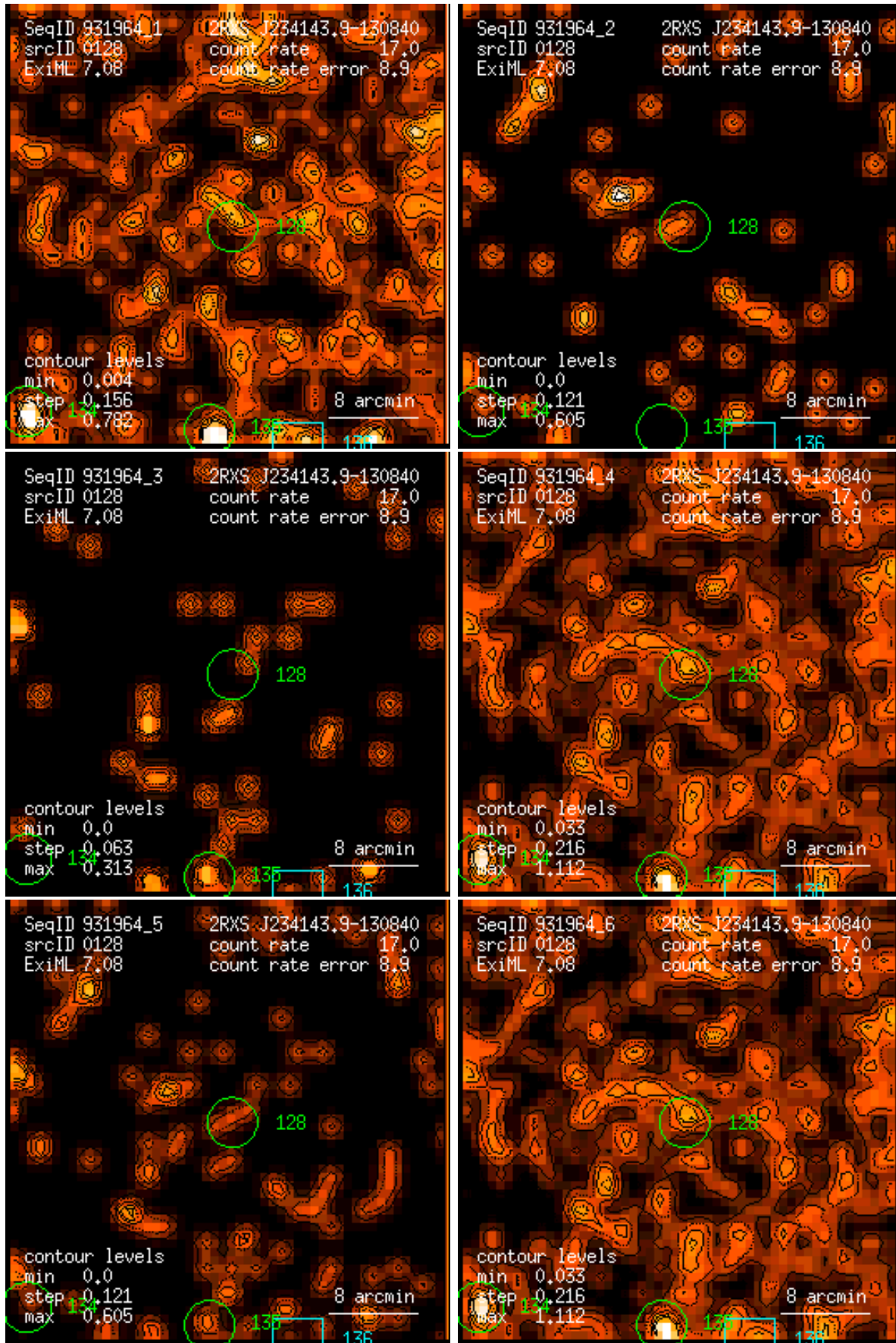
Figure 128: RASS 931964: detection 0128: band rate images, Gaussian filter: (1) PSPC channels 11 – 41, (2) 52 – 90, (3) 91 – 201, (4) 11 – 235, (5) 52 – 201, (6) 11 – 201. Broad band rates in counts/ks. Band rate contour levels in counts/ks/arcmin 2 .
