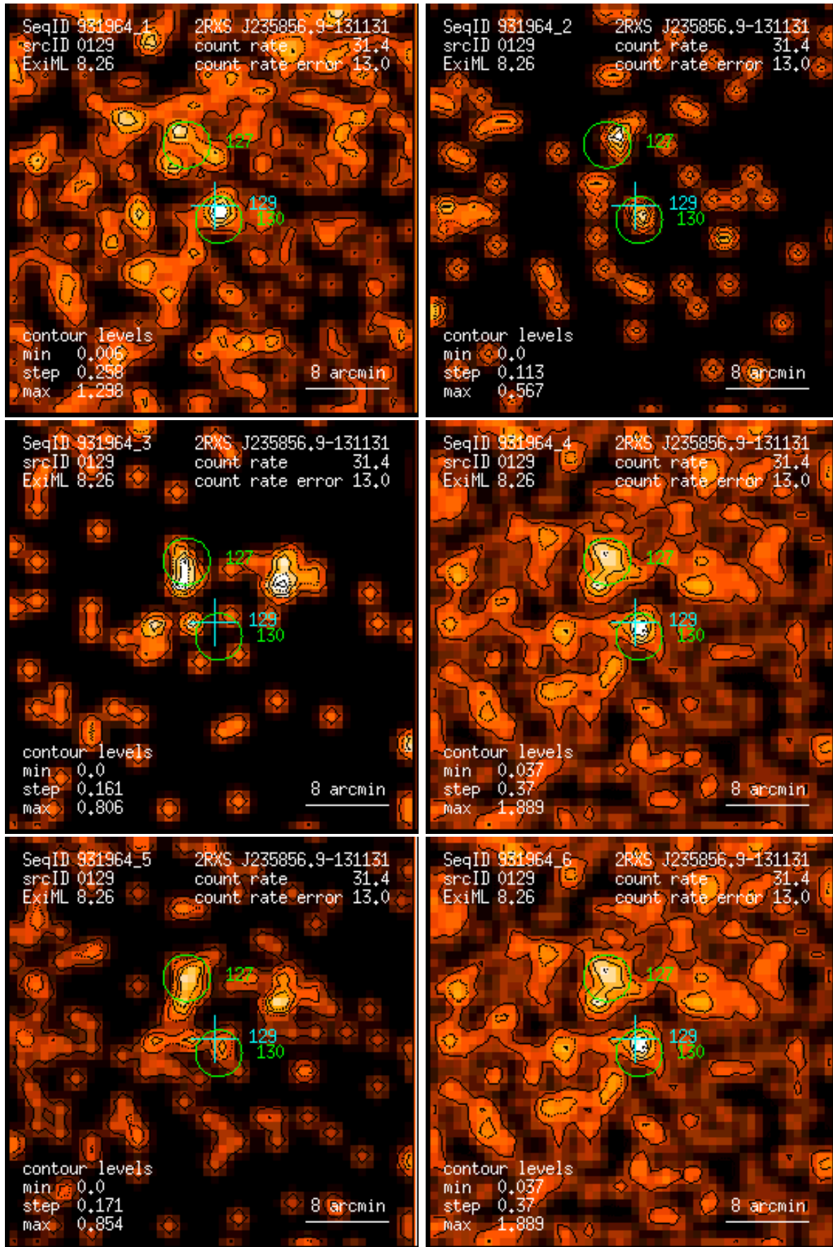
Figure 129: RASS 931964: detection 0129: band rate images, Gaussian filter: (1) PSPC channels 11 – 41, (2) 52 – 90, (3) 91 – 201, (4) 11 – 235, (5) 52 – 201, (6) 11 – 201. Broad band rates in counts/ks. Band rate contour levels in counts/ks/arcmin 2 .
