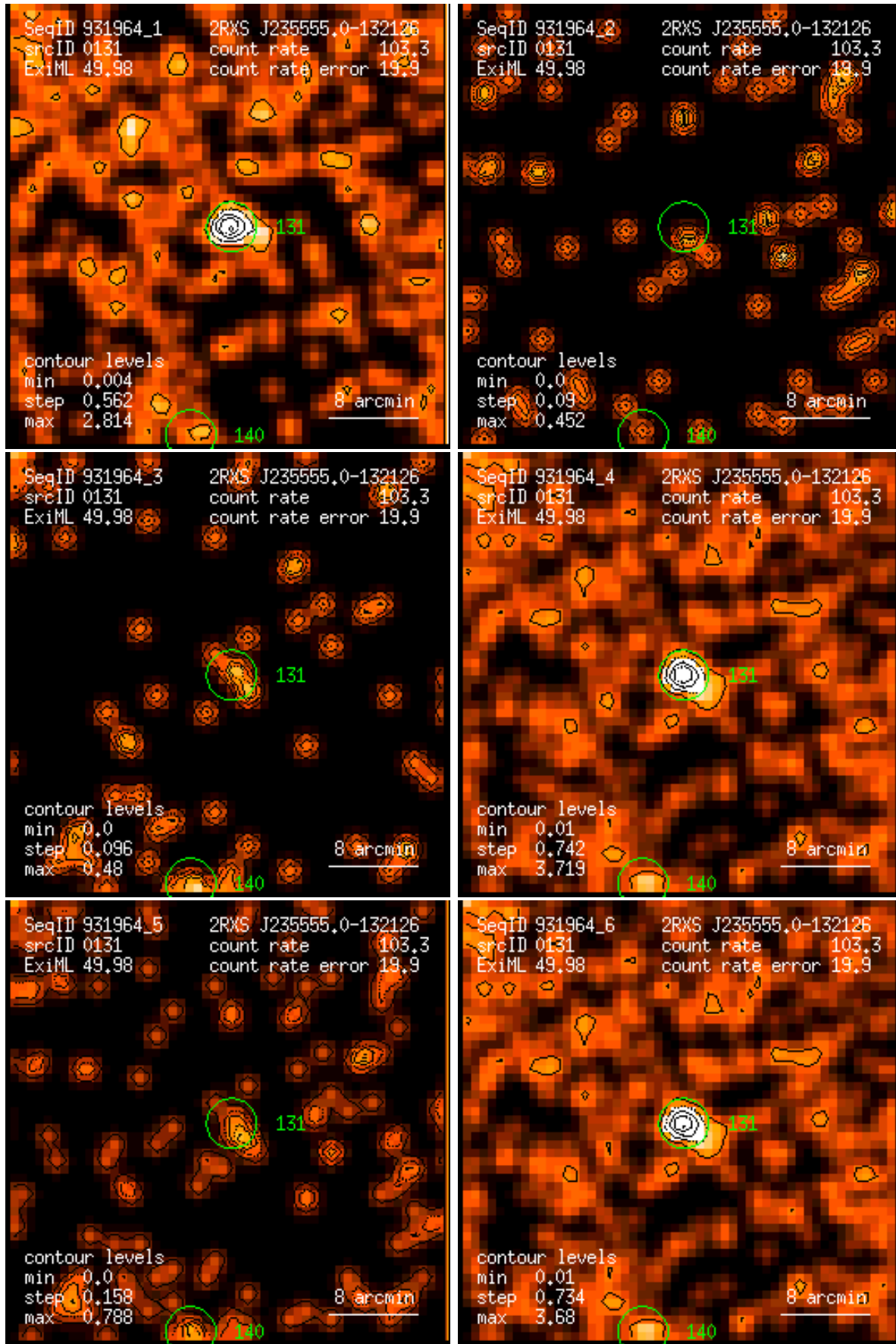
Figure 131: RASS 931964: detection 0131: band rate images, Gaussian filter: (1) PSPC channels 11 – 41, (2) 52 – 90, (3) 91 – 201, (4) 11 – 235, (5) 52 – 201, (6) 11 – 201. Broad band rates in counts/ks. Band rate contour levels in counts/ks/arcmin 2 .
