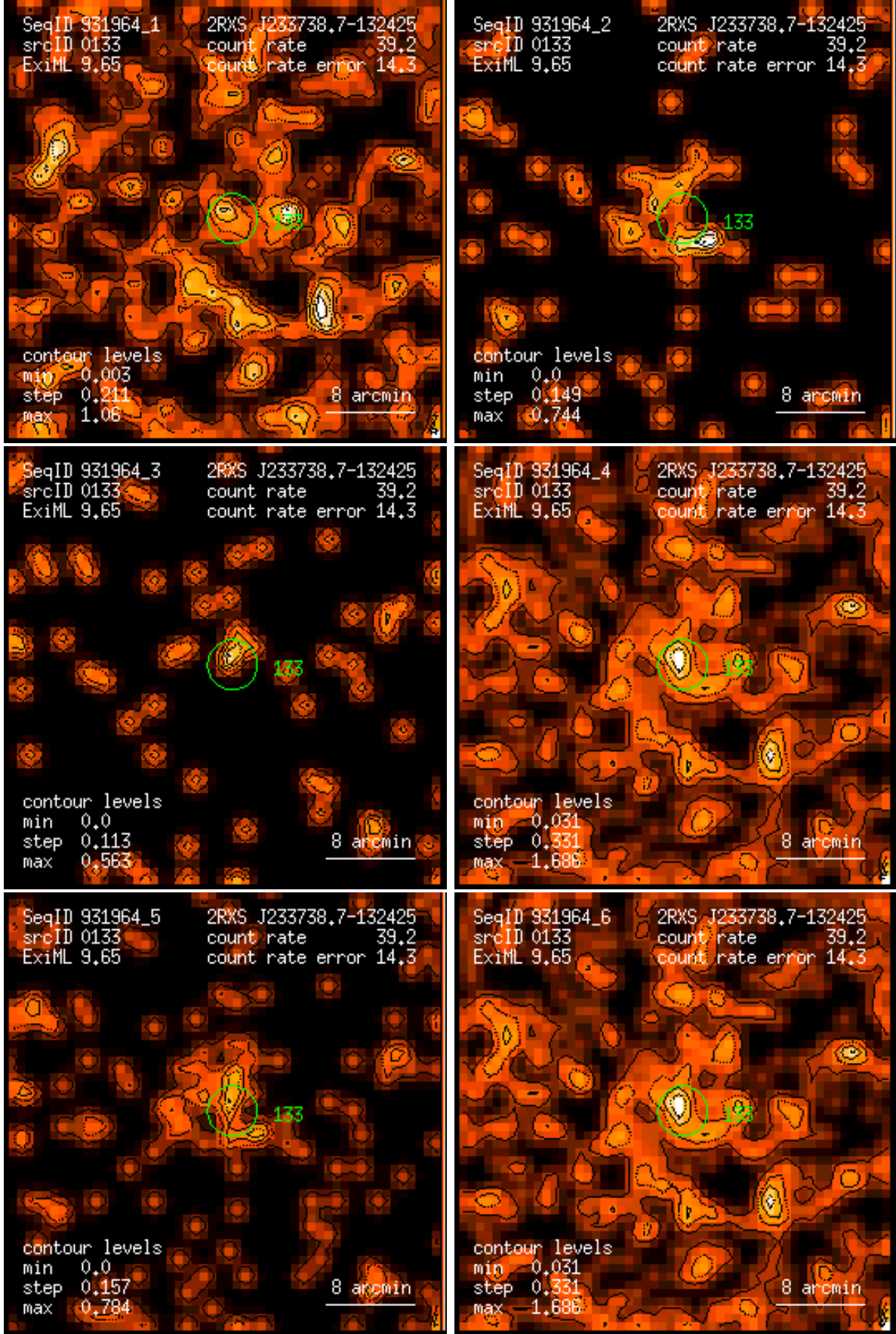
Figure 133: RASS 931964: detection 0133: band rate images, Gaussian filter: (1) PSPC channels 11 – 41, (2) 52 – 90, (3) 91 – 201, (4) 11 – 235, (5) 52 – 201, (6) 11 – 201. Broad band rates in counts/ks. Band rate contour levels in counts/ks/arcmin 2 .
