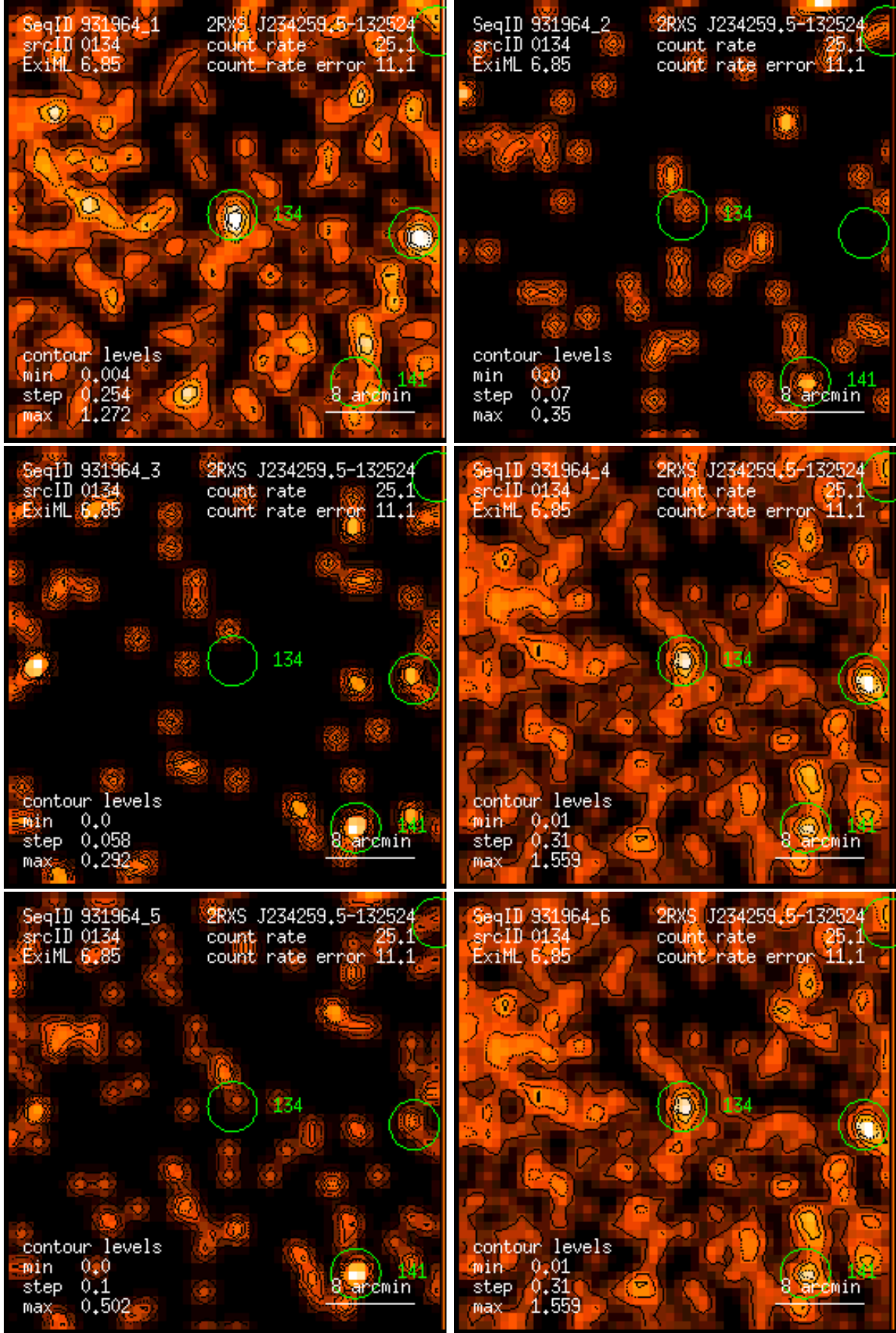
Figure 134: RASS 931964: detection 0134: band rate images, Gaussian filter: (1) PSPC channels 11 – 41, (2) 52 – 90, (3) 91 – 201, (4) 11 – 235, (5) 52 – 201, (6) 11 – 201. Broad band rates in counts/ks. Band rate contour levels in counts/ks/arcmin 2 .
