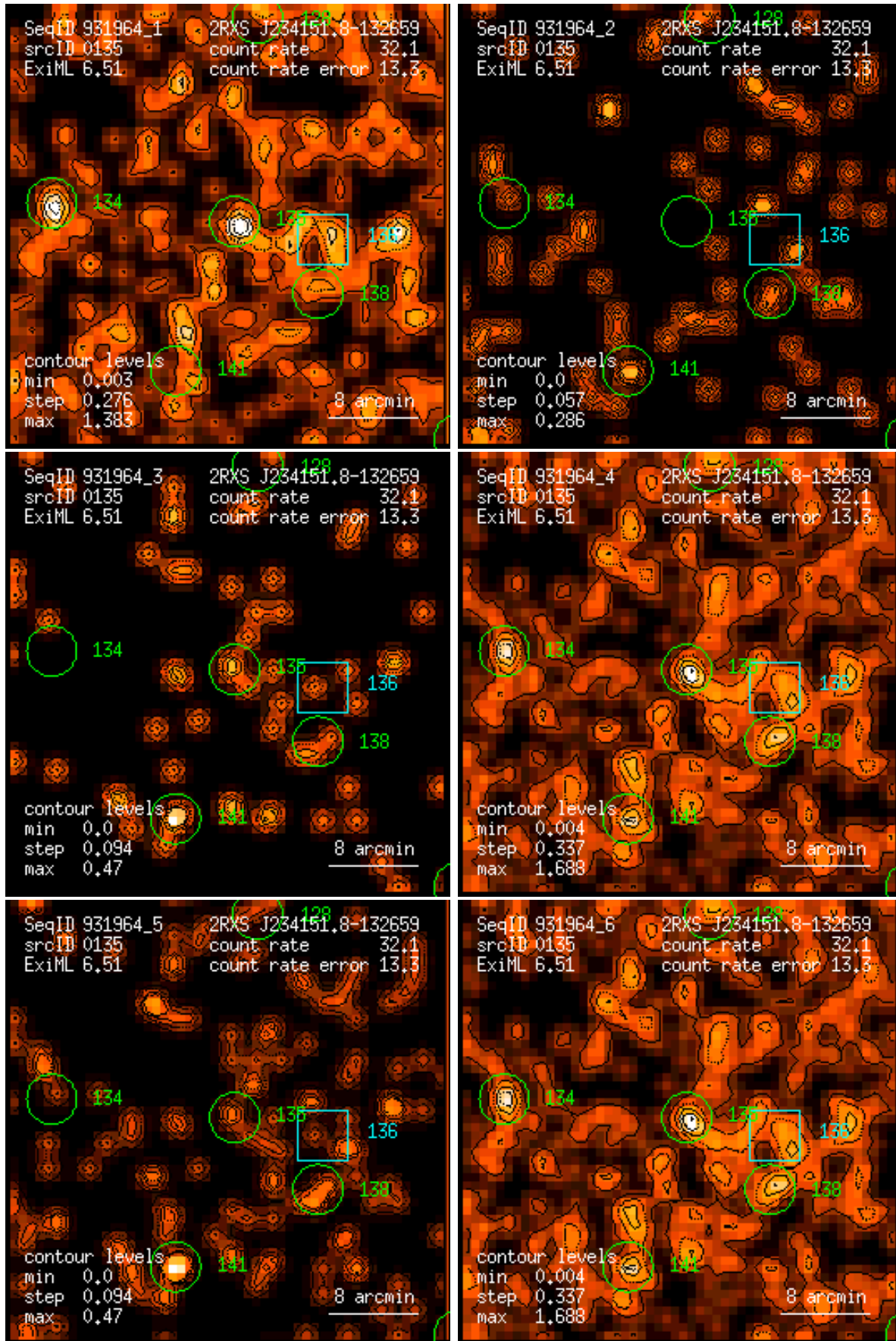
Figure 135: RASS 931964: detection 0135: band rate images, Gaussian filter: (1) PSPC channels 11 – 41, (2) 52 – 90, (3) 91 – 201, (4) 11 – 235, (5) 52 – 201, (6) 11 – 201. Broad band rates in counts/ks. Band rate contour levels in counts/ks/arcmin 2 .
