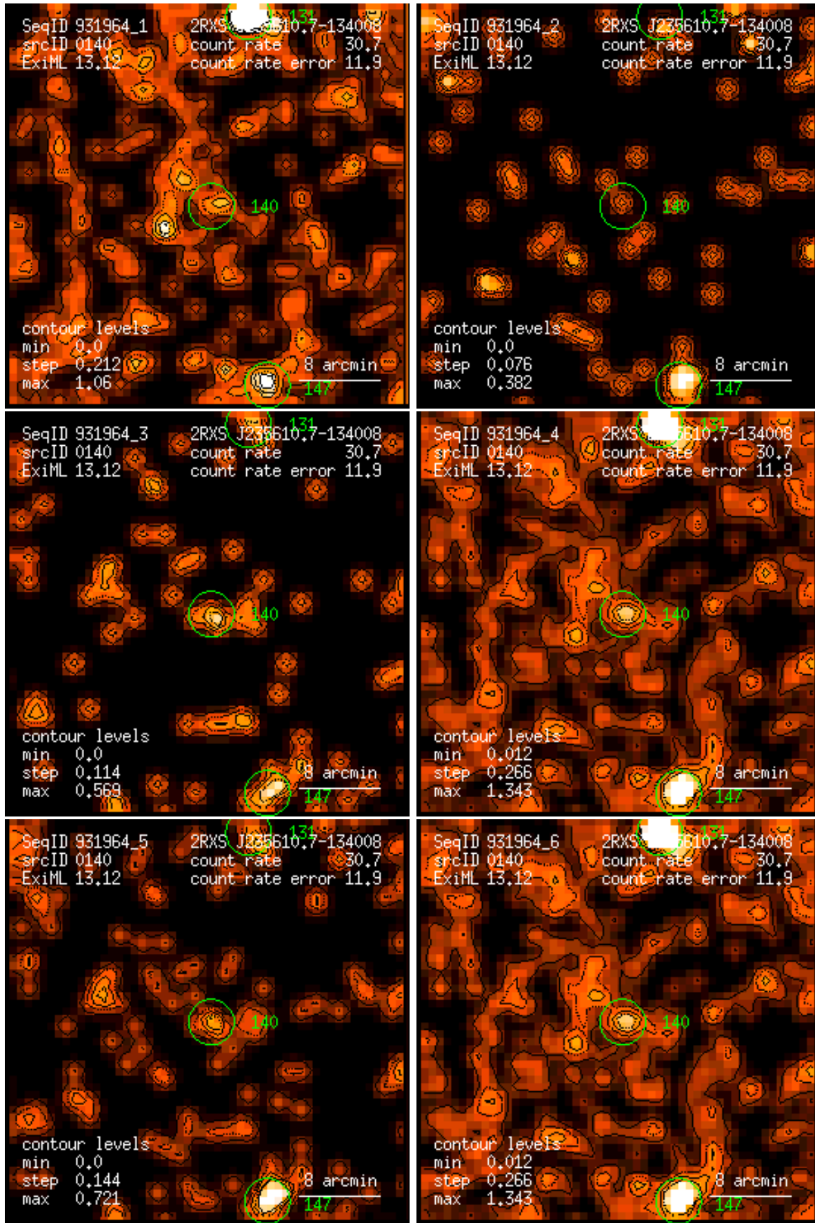
Figure 140: RASS 931964: detection 0140: band rate images, Gaussian filter: (1) PSPC channels 11 – 41, (2) 52 – 90, (3) 91 – 201, (4) 11 – 235, (5) 52 – 201, (6) 11 – 201. Broad band rates in counts/ks. Band rate contour levels in counts/ks/arcmin 2 .
