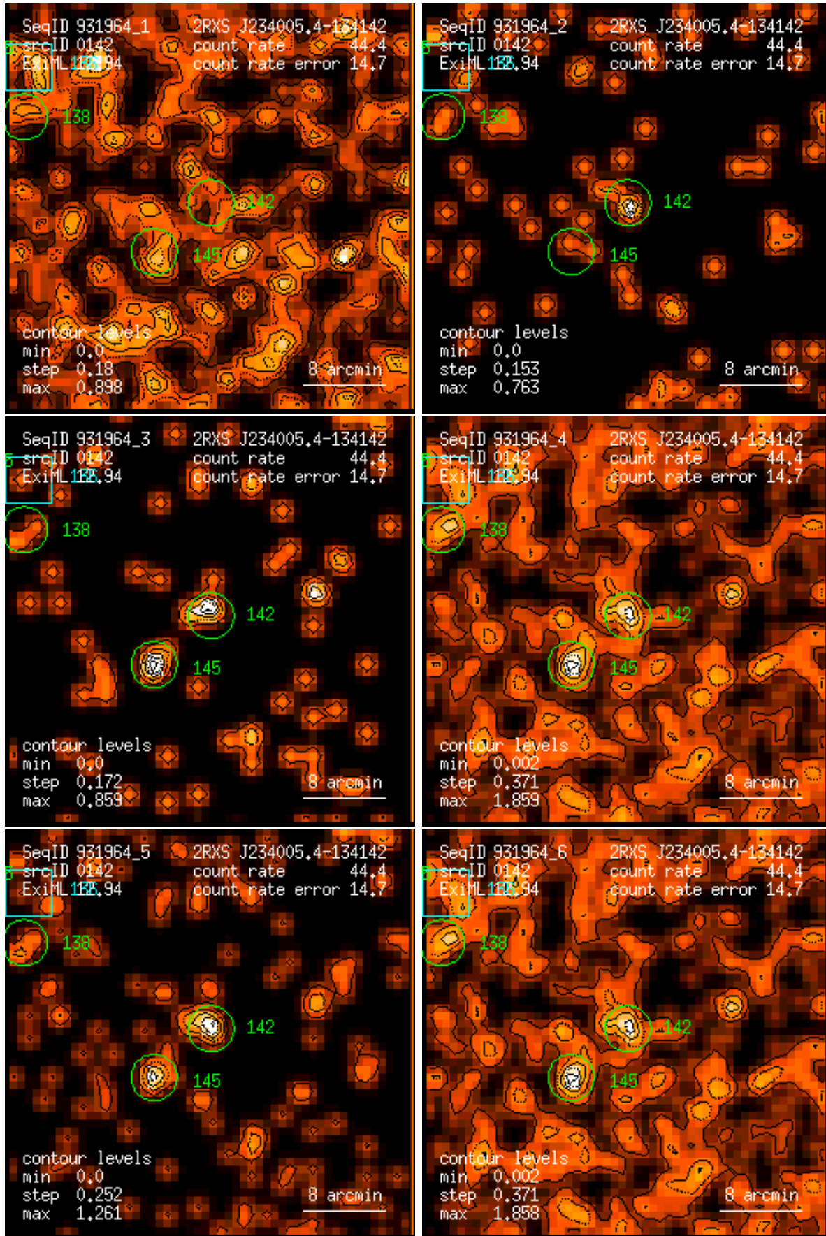
Figure 142: RASS 931964: detection 0142: band rate images, Gaussian filter: (1) PSPC channels 11 – 41, (2) 52 – 90, (3) 91 – 201, (4) 11 – 235, (5) 52 – 201, (6) 11 – 201. Broad band rates in counts/ks. Band rate contour levels in counts/ks/arcmin 2 .
