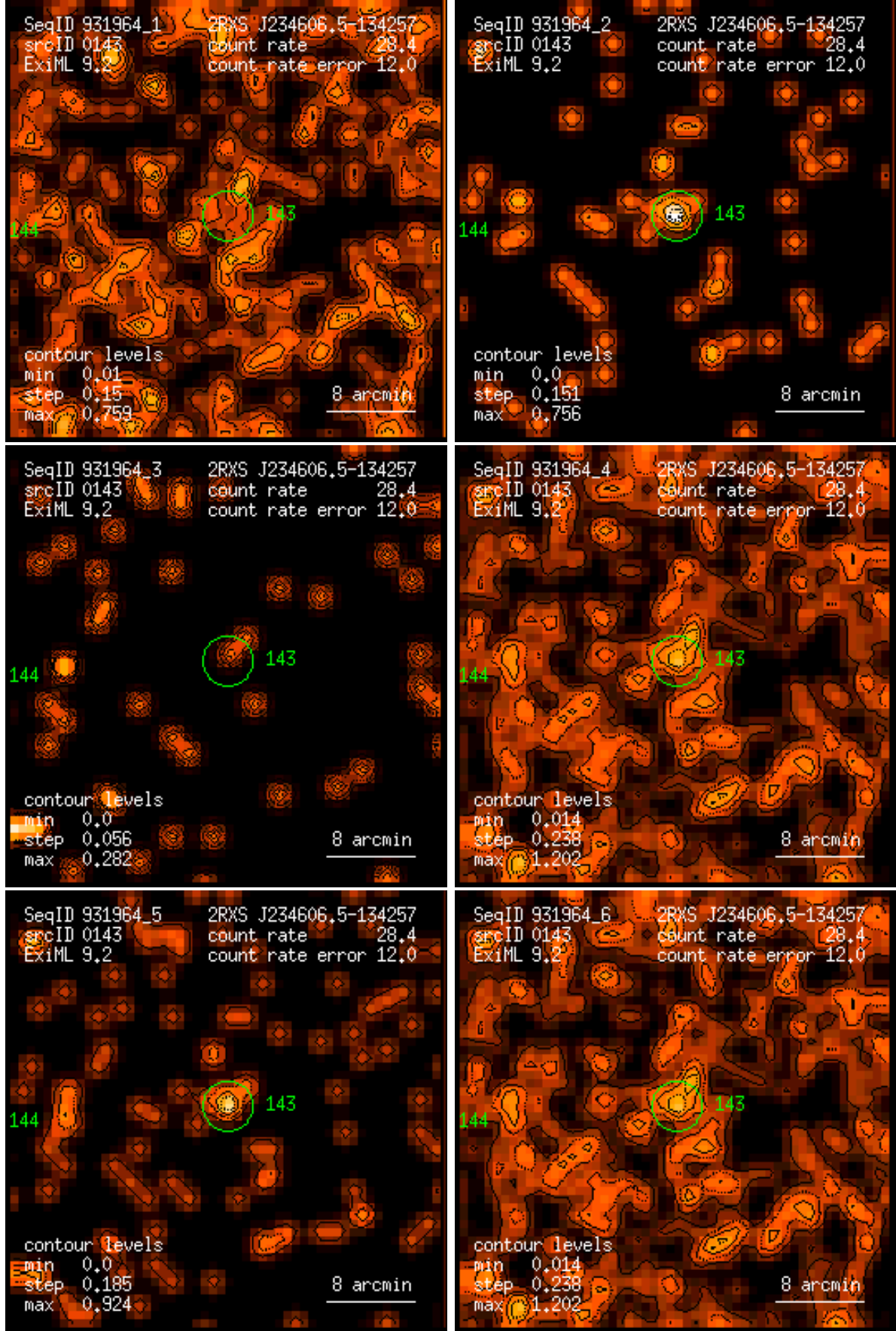
Figure 143: RASS 931964: detection 0143: band rate images, Gaussian filter: (1) PSPC channels 11 – 41, (2) 52 – 90, (3) 91 – 201, (4) 11 – 235, (5) 52 – 201, (6) 11 – 201. Broad band rates in counts/ks. Band rate contour levels in counts/ks/arcmin 2 .
