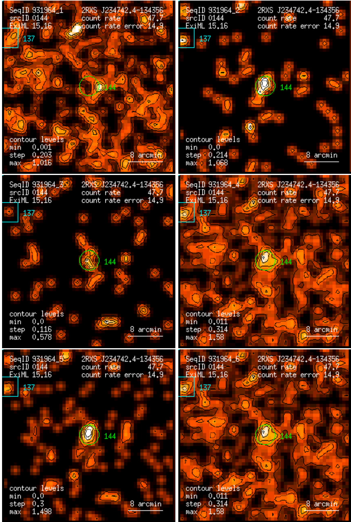
Figure 144: RASS 931964: detection 0144: band rate images, Gaussian filter: (1) PSPC channels 11 – 41, (2) 52 – 90, (3) 91 – 201, (4) 11 – 235, (5) 52 – 201, (6) 11 – 201. Broad band rates in counts/ks. Band rate contour levels in counts/ks/arcmin 2 .
