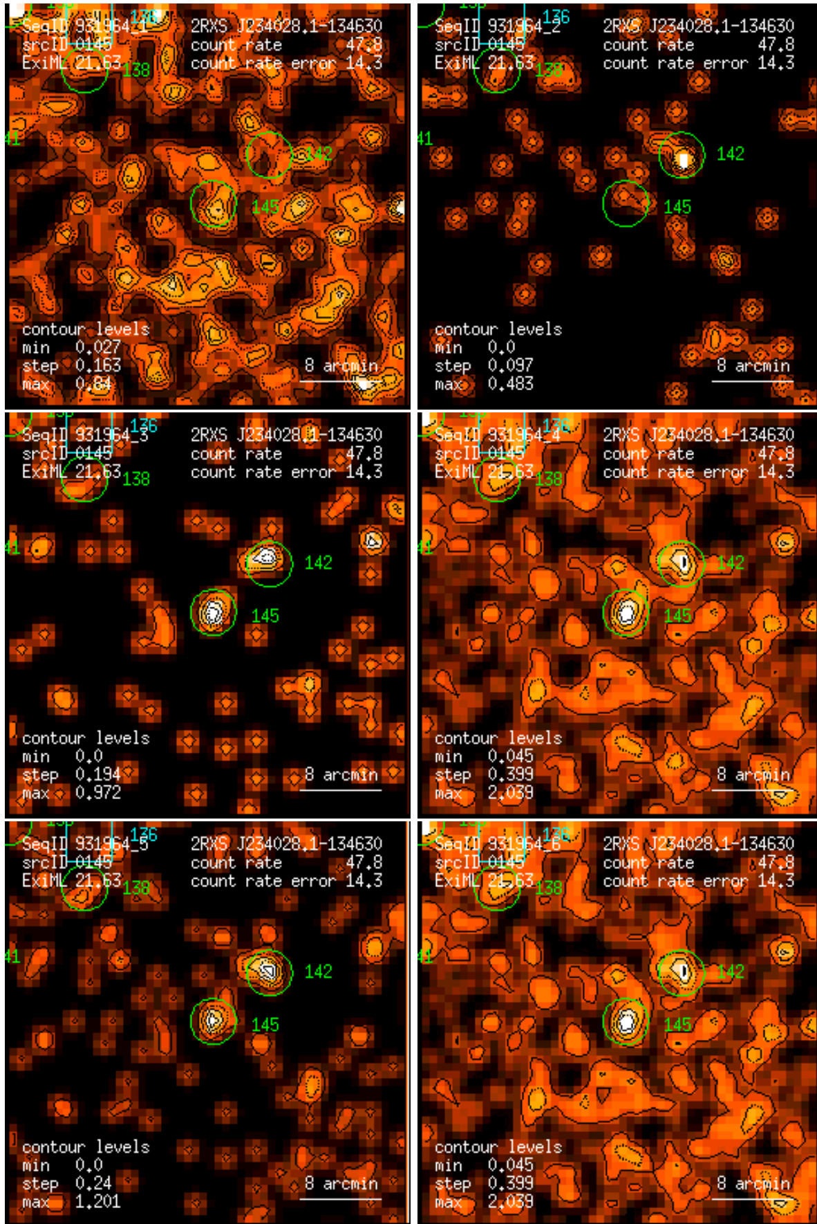
Figure 145: RASS 931964: detection 0145: band rate images, Gaussian filter: (1) PSPC channels 11 – 41, (2) 52 – 90, (3) 91 – 201, (4) 11 – 235, (5) 52 – 201, (6) 11 – 201. Broad band rates in counts/ks. Band rate contour levels in counts/ks/arcmin 2 .
