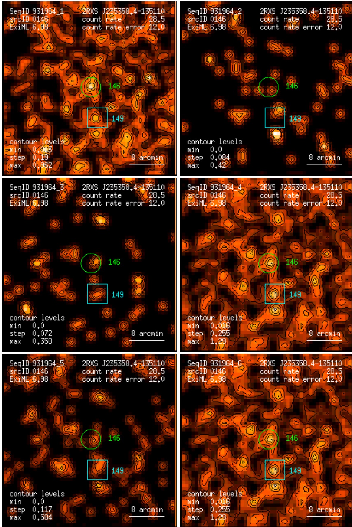
Figure 146: RASS 931964: detection 0146: band rate images, Gaussian filter: (1) PSPC channels 11 – 41, (2) 52 – 90, (3) 91 – 201, (4) 11 – 235, (5) 52 – 201, (6) 11 – 201. Broad band rates in counts/ks. Band rate contour levels in counts/ks/arcmin 2 .
