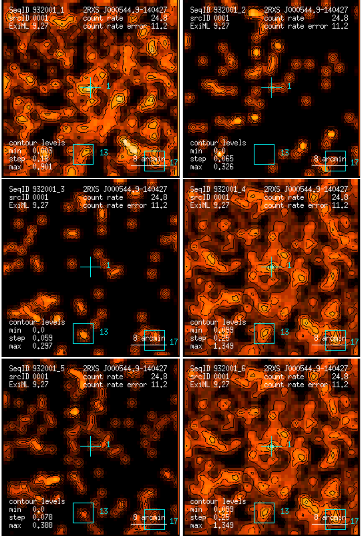
Figure 1: RASS 932001: detection 0001: band rate images, Gaussian filter: (1) PSPC channels 11 – 41, (2) 52 – 90, (3) 91 – 201, (4) 11 – 235, (5) 52 – 201, (6) 11 – 201. Broad band rates in counts/ks. Band rate contour levels in counts/ks/arcmin 2 .
