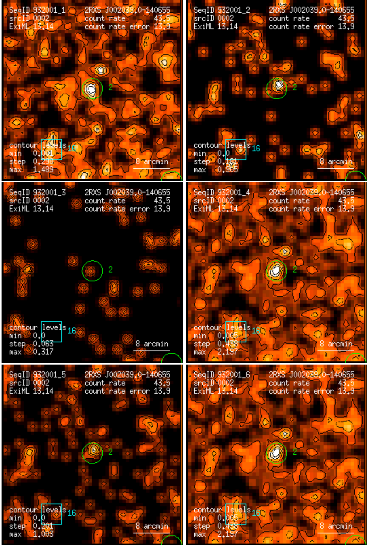
Figure 2: RASS 932001: detection 0002: band rate images, Gaussian filter: (1) PSPC channels 11 – 41, (2) 52 – 90, (3) 91 – 201, (4) 11 – 235, (5) 52 – 201, (6) 11 – 201. Broad band rates in counts/ks. Band rate contour levels in counts/ks/arcmin 2 .
