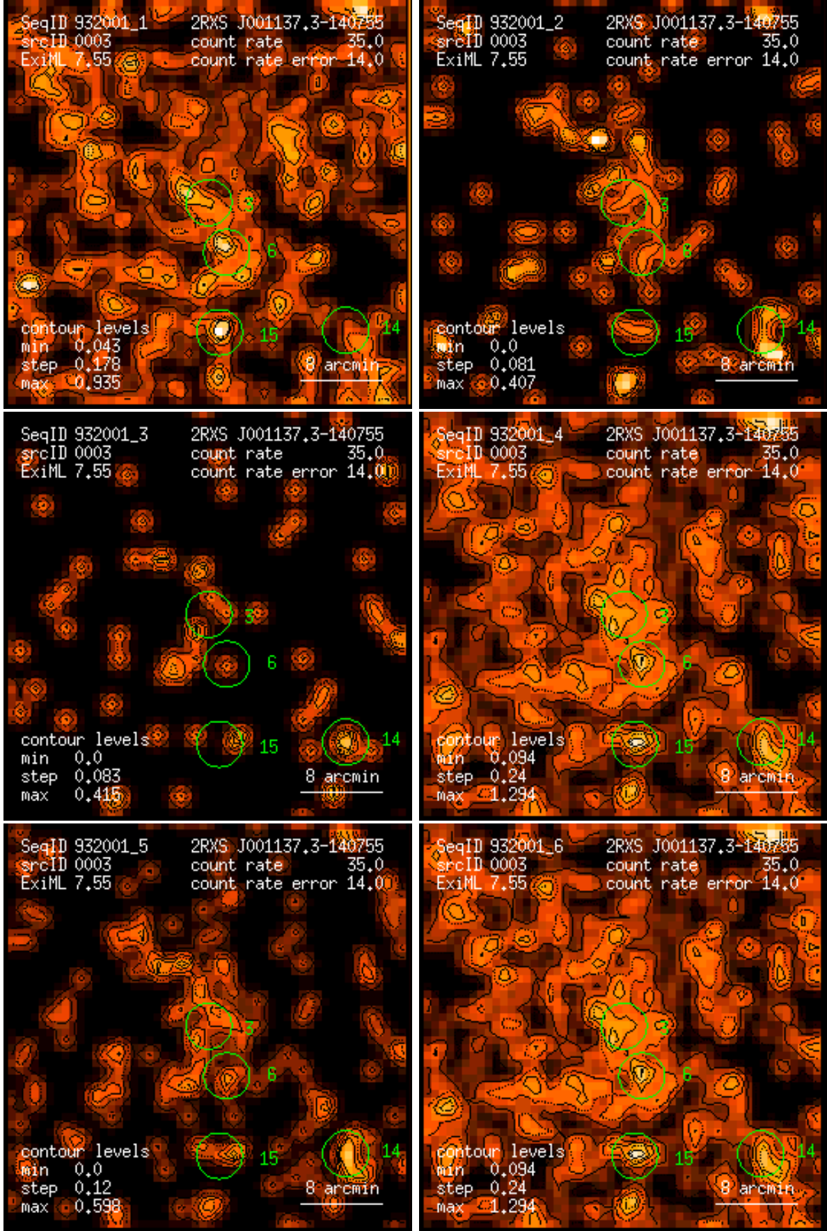
Figure 3: RASS 932001: detection 0003: band rate images, Gaussian filter: (1) PSPC channels 11 – 41, (2) 52 – 90, (3) 91 – 201, (4) 11 – 235, (5) 52 – 201, (6) 11 – 201. Broad band rates in counts/ks. Band rate contour levels in counts/ks/arcmin 2 .
