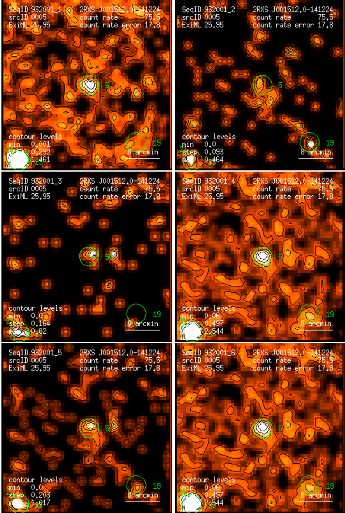
Figure 5: RASS 932001: detection 0005: band rate images, Gaussian filter: (1) PSPC channels 11 – 41, (2) 52 – 90, (3) 91 – 201, (4) 11 – 235, (5) 52 – 201, (6) 11 – 201. Broad band rates in counts/ks. Band rate contour levels in counts/ks/arcmin 2 .
