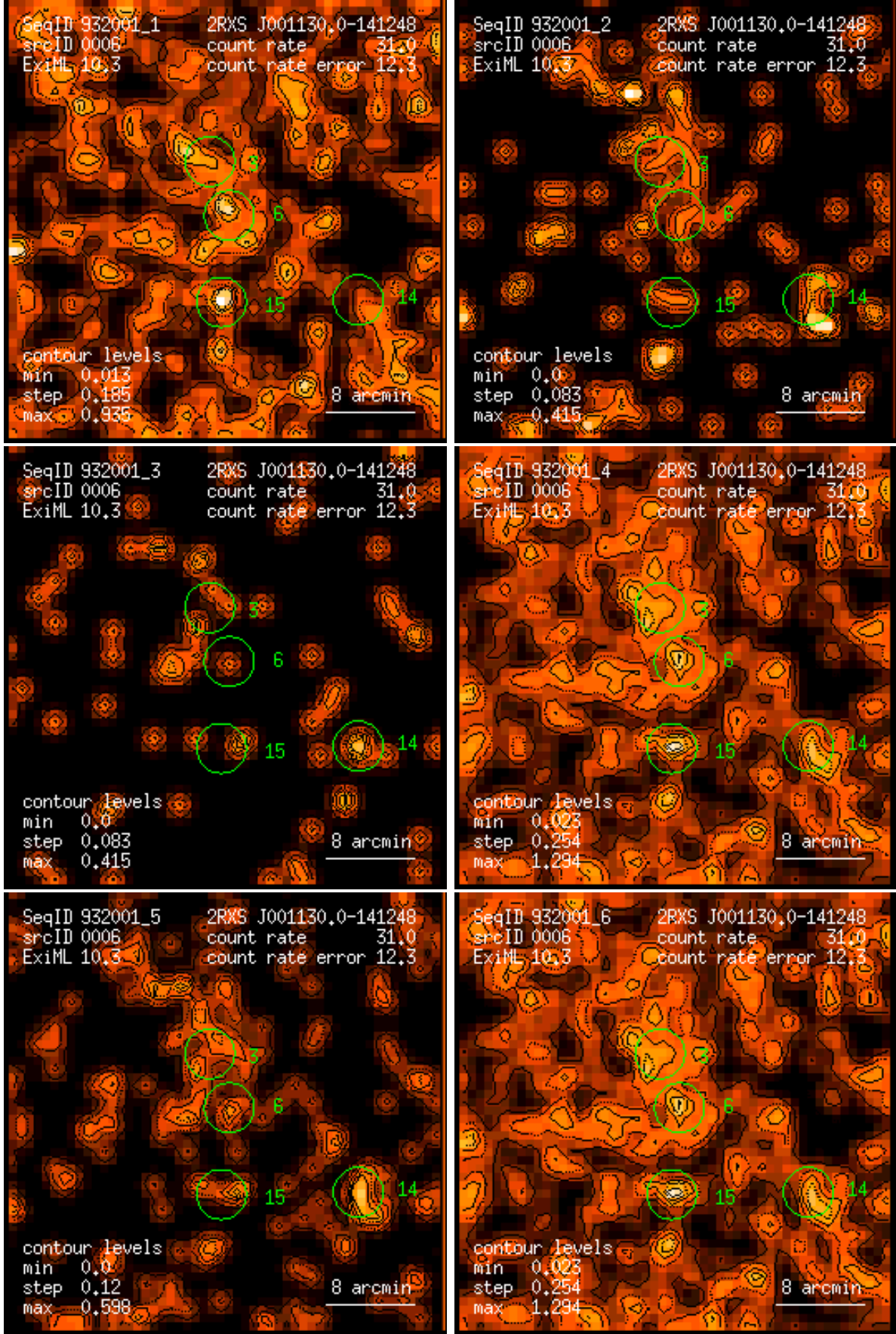
Figure 6: RASS 932001: detection 0006: band rate images, Gaussian filter: (1) PSPC channels 11 – 41, (2) 52 – 90, (3) 91 – 201, (4) 11 – 235, (5) 52 – 201, (6) 11 – 201. Broad band rates in counts/ks. Band rate contour levels in counts/ks/arcmin 2 .
