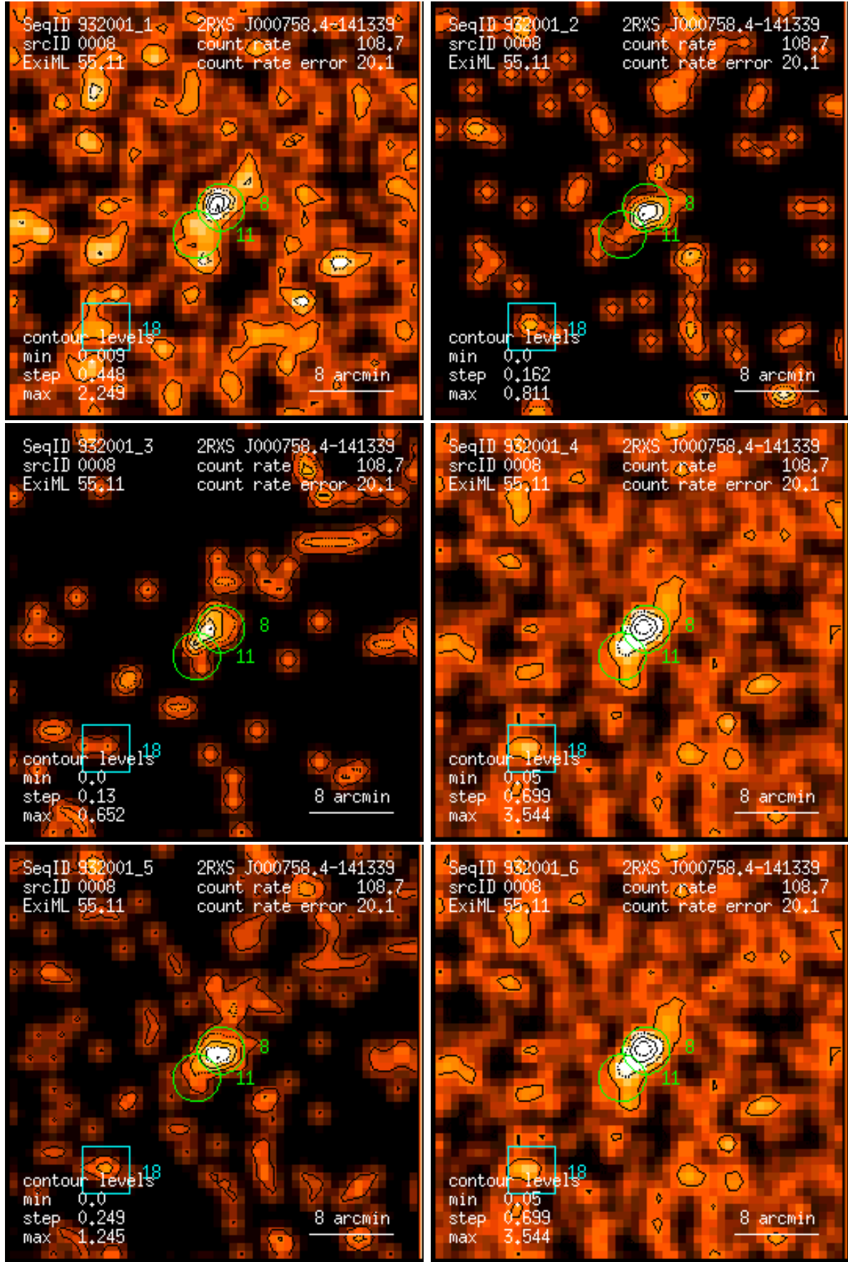
Figure 8: RASS 932001: detection 0008: band rate images, Gaussian filter: (1) PSPC channels 11 – 41, (2) 52 – 90, (3) 91 – 201, (4) 11 – 235, (5) 52 – 201, (6) 11 – 201. Broad band rates in counts/ks. Band rate contour levels in counts/ks/arcmin 2 .
