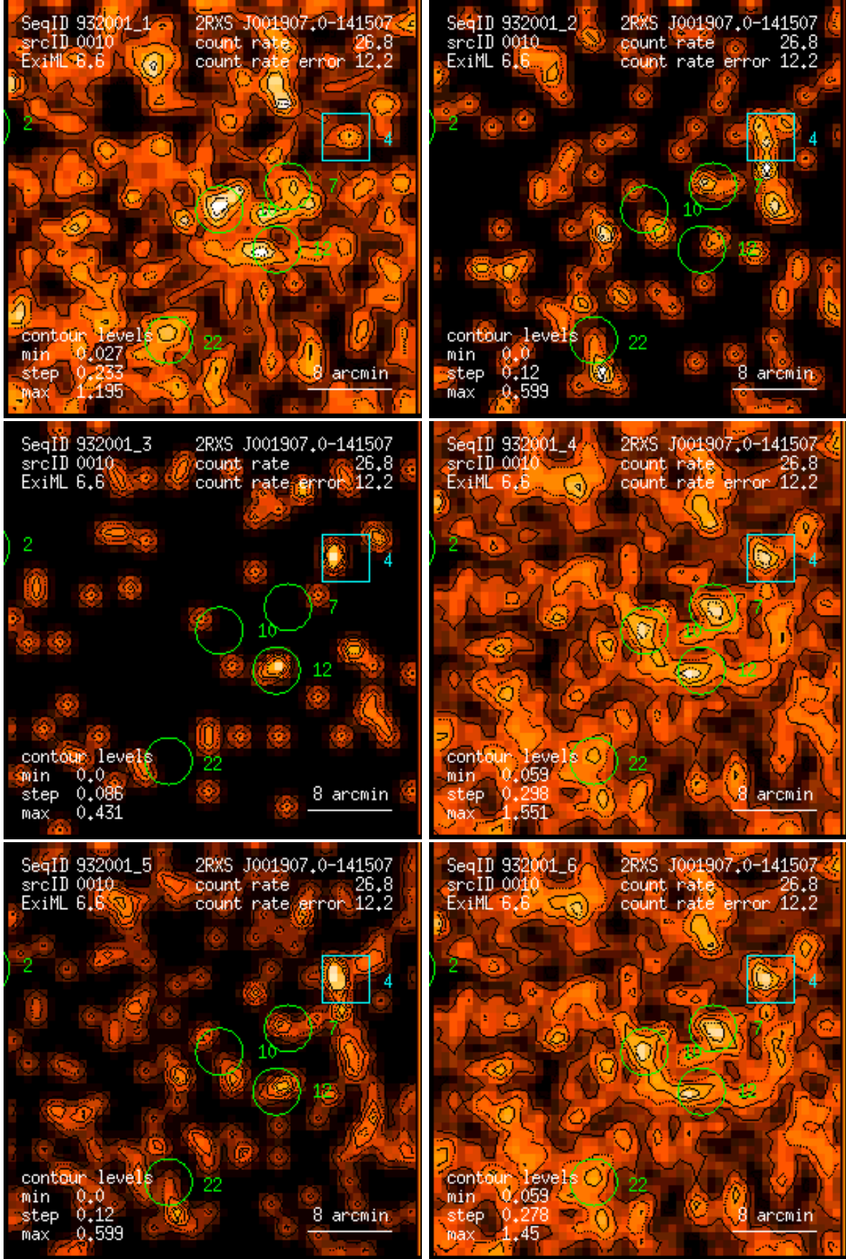
Figure 10: RASS 932001: detection 0010: band rate images, Gaussian filter: (1) PSPC channels 11 – 41, (2) 52 – 90, (3) 91 – 201, (4) 11 – 235, (5) 52 – 201, (6) 11 – 201. Broad band rates in counts/ks. Band rate contour levels in counts/ks/arcmin 2 .
