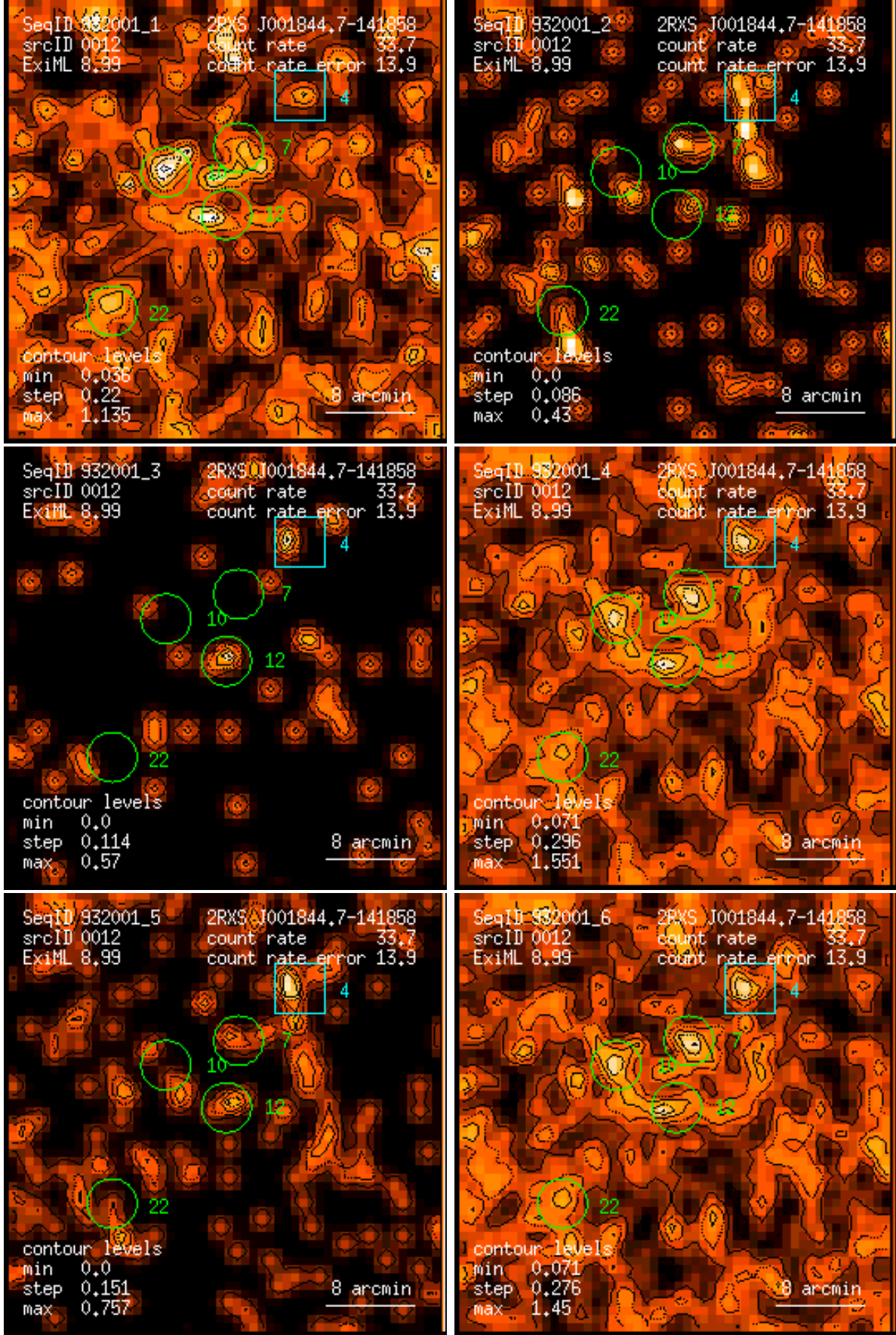
Figure 12: RASS 932001: detection 0012: band rate images, Gaussian filter: (1) PSPC channels 11 – 41, (2) 52 – 90, (3) 91 – 201, (4) 11 – 235, (5) 52 – 201, (6) 11 – 201. Broad band rates in counts/ks. Band rate contour levels in counts/ks/arcmin 2 .
