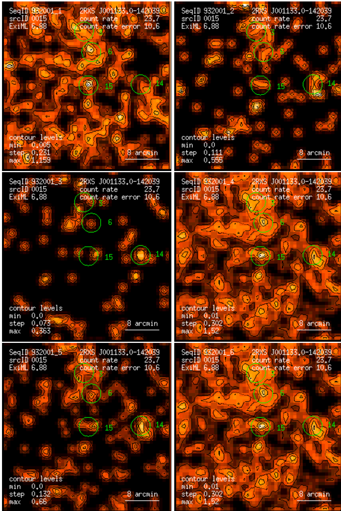
Figure 15: RASS 932001: detection 0015: band rate images, Gaussian filter: (1) PSPC channels 11 – 41, (2) 52 – 90, (3) 91 – 201, (4) 11 – 235, (5) 52 – 201, (6) 11 – 201. Broad band rates in counts/ks. Band rate contour levels in counts/ks/arcmin 2 .
