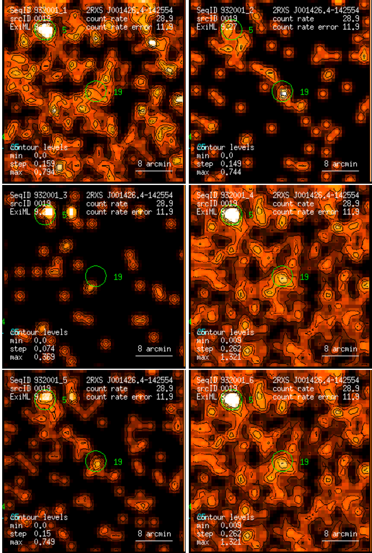
Figure 19: RASS 932001: detection 0019: band rate images, Gaussian filter: (1) PSPC channels 11 – 41, (2) 52 – 90, (3) 91 – 201, (4) 11 – 235, (5) 52 – 201, (6) 11 – 201. Broad band rates in counts/ks. Band rate contour levels in counts/ks/arcmin 2 .
