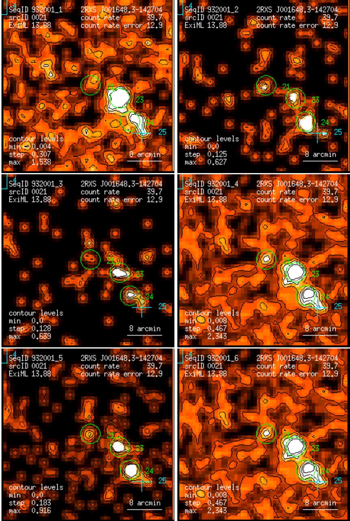
Figure 21: RASS 932001: detection 0021: band rate images, Gaussian filter: (1) PSPC channels 11 – 41, (2) 52 – 90, (3) 91 – 201, (4) 11 – 235, (5) 52 – 201, (6) 11 – 201. Broad band rates in counts/ks. Band rate contour levels in counts/ks/arcmin 2 .
