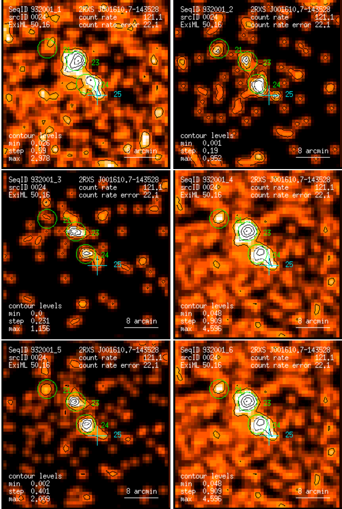
Figure 24: RASS 932001: detection 0024: band rate images, Gaussian filter: (1) PSPC channels 11 – 41, (2) 52 – 90, (3) 91 – 201, (4) 11 – 235, (5) 52 – 201, (6) 11 – 201. Broad band rates in counts/ks. Band rate contour levels in counts/ks/arcmin 2 .
