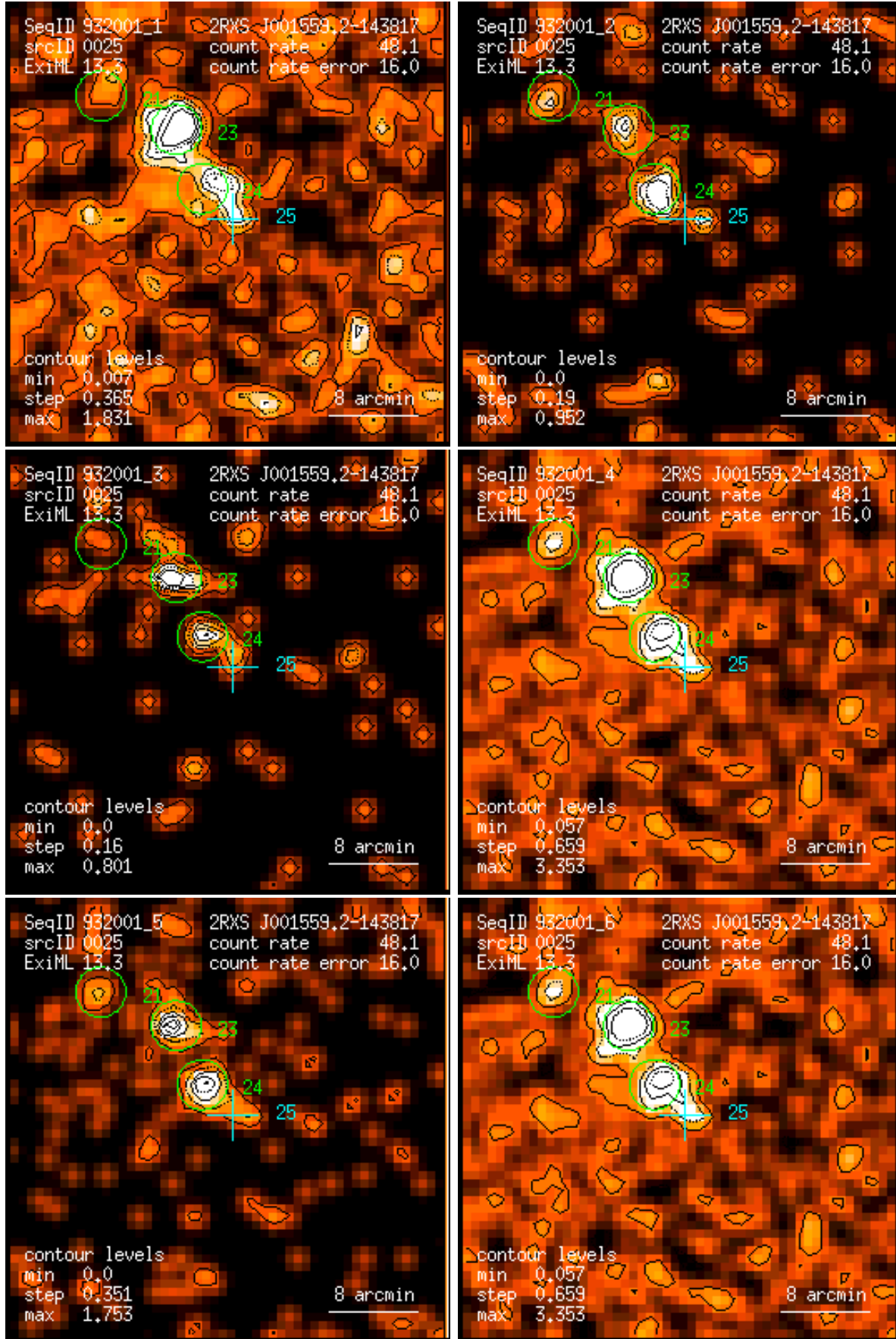
Figure 25: RASS 932001: detection 0025: band rate images, Gaussian filter: (1) PSPC channels 11 – 41, (2) 52 – 90, (3) 91 – 201, (4) 11 – 235, (5) 52 – 201, (6) 11 – 201. Broad band rates in counts/ks. Band rate contour levels in counts/ks/arcmin 2 .
