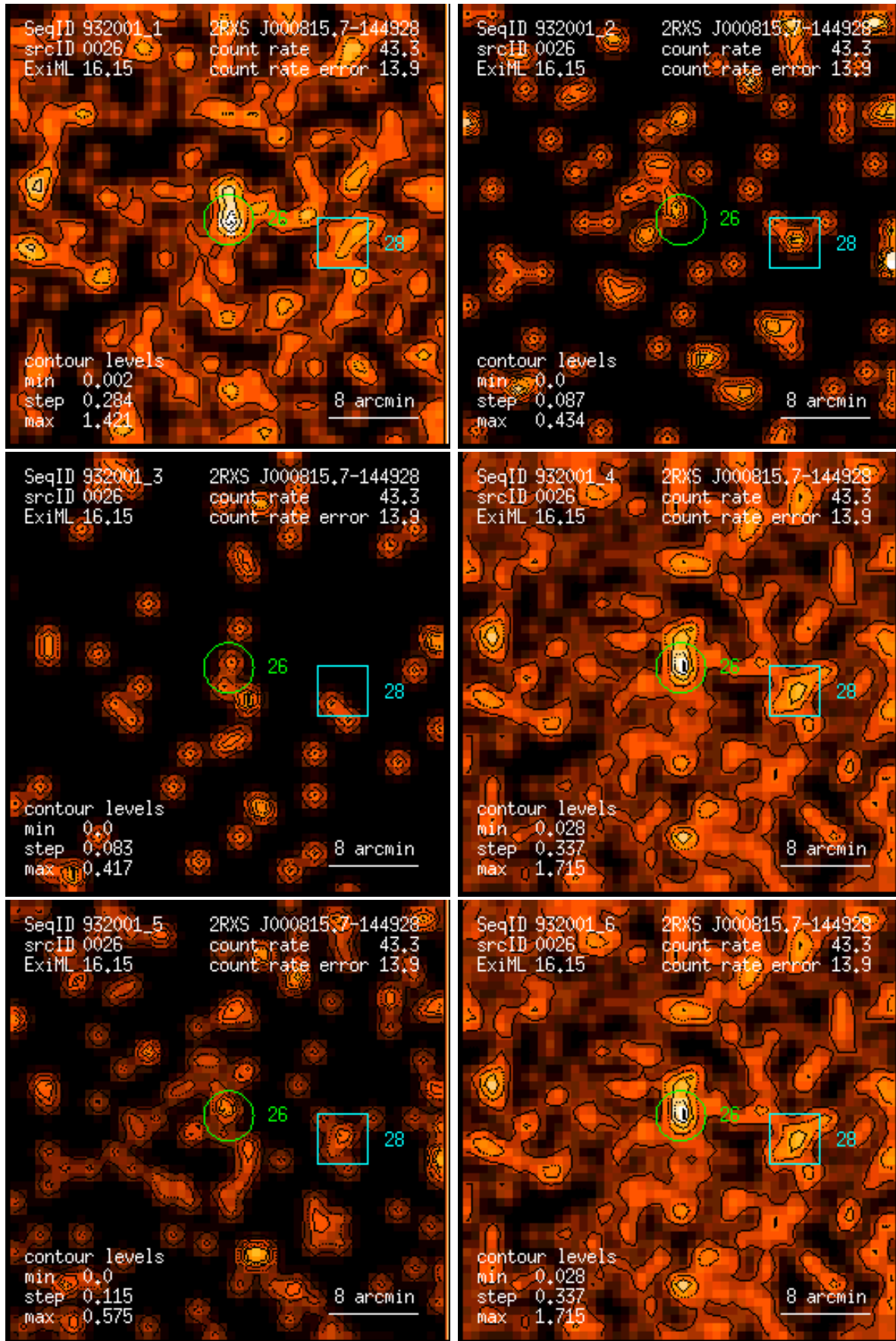
Figure 26: RASS 932001: detection 0026: band rate images, Gaussian filter: (1) PSPC channels 11 – 41, (2) 52 – 90, (3) 91 – 201, (4) 11 – 235, (5) 52 – 201, (6) 11 – 201. Broad band rates in counts/ks. Band rate contour levels in counts/ks/arcmin 2 .
