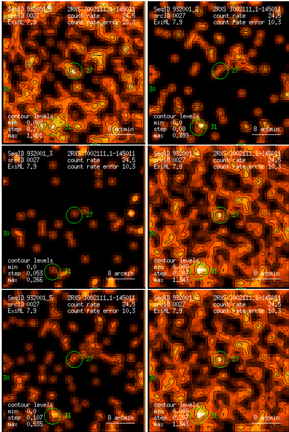
Figure 27: RASS 932001: detection 0027: band rate images, Gaussian filter: (1) PSPC channels 11 – 41, (2) 52 – 90, (3) 91 – 201, (4) 11 – 235, (5) 52 – 201, (6) 11 – 201. Broad band rates in counts/ks. Band rate contour levels in counts/ks/arcmin 2 .
