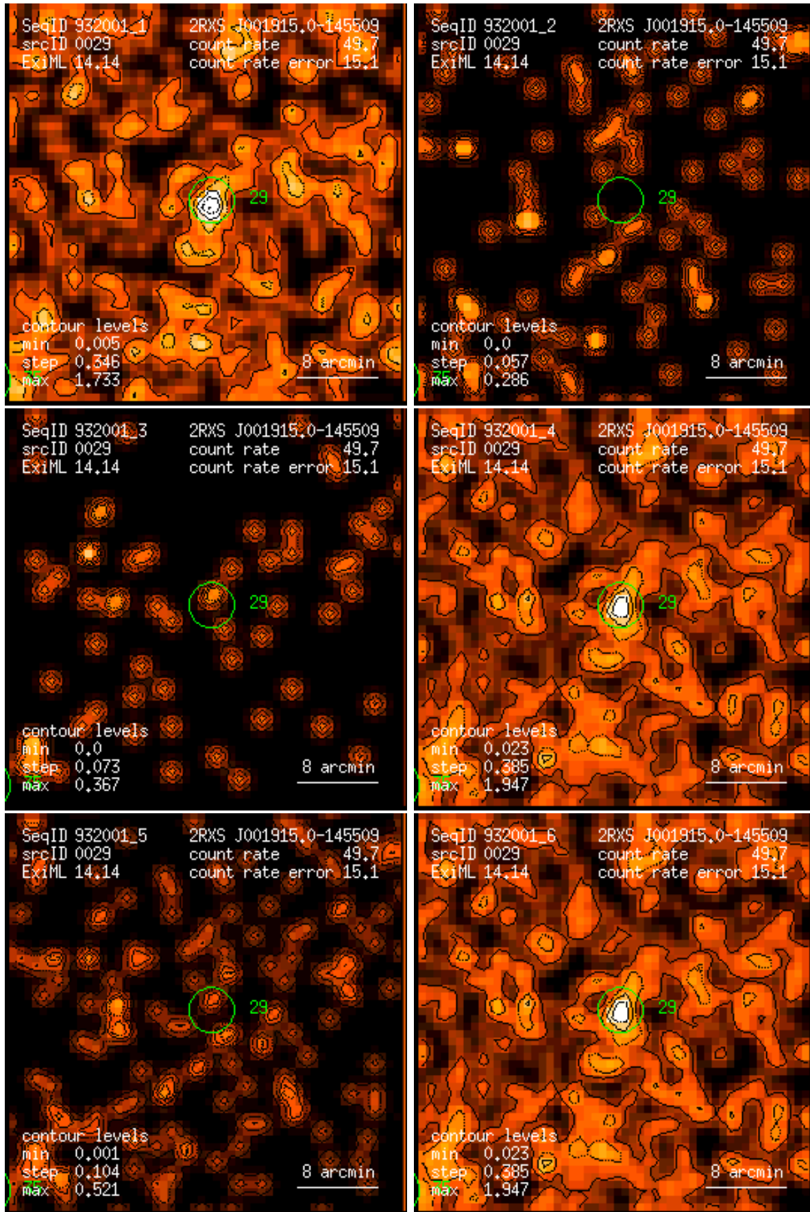
Figure 29: RASS 932001: detection 0029: band rate images, Gaussian filter: (1) PSPC channels 11 – 41, (2) 52 – 90, (3) 91 – 201, (4) 11 – 235, (5) 52 – 201, (6) 11 – 201. Broad band rates in counts/ks. Band rate contour levels in counts/ks/arcmin 2 .
