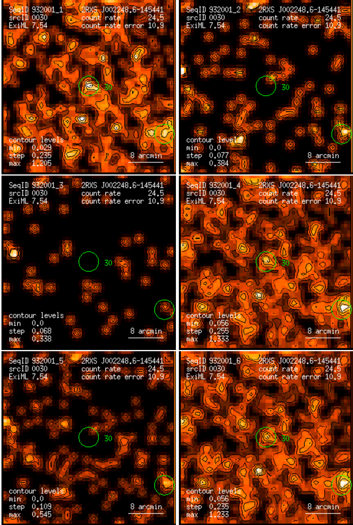
Figure 30: RASS 932001: detection 0030: band rate images, Gaussian filter: (1) PSPC channels 11 – 41, (2) 52 – 90, (3) 91 – 201, (4) 11 – 235, (5) 52 – 201, (6) 11 – 201. Broad band rates in counts/ks. Band rate contour levels in counts/ks/arcmin 2 .
