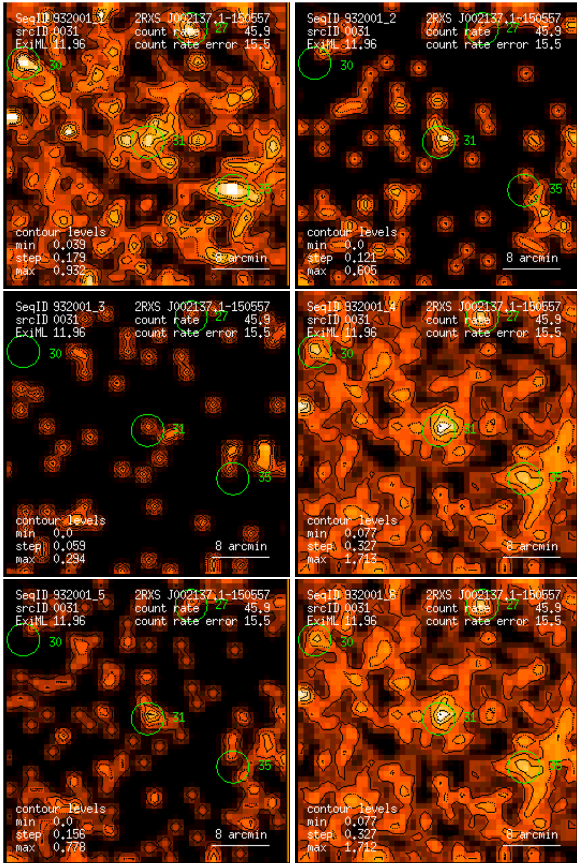
Figure 31: RASS 932001: detection 0031: band rate images, Gaussian filter: (1) PSPC channels 11 – 41, (2) 52 – 90, (3) 91 – 201, (4) 11 – 235, (5) 52 – 201, (6) 11 – 201. Broad band rates in counts/ks. Band rate contour levels in counts/ks/arcmin 2 .
