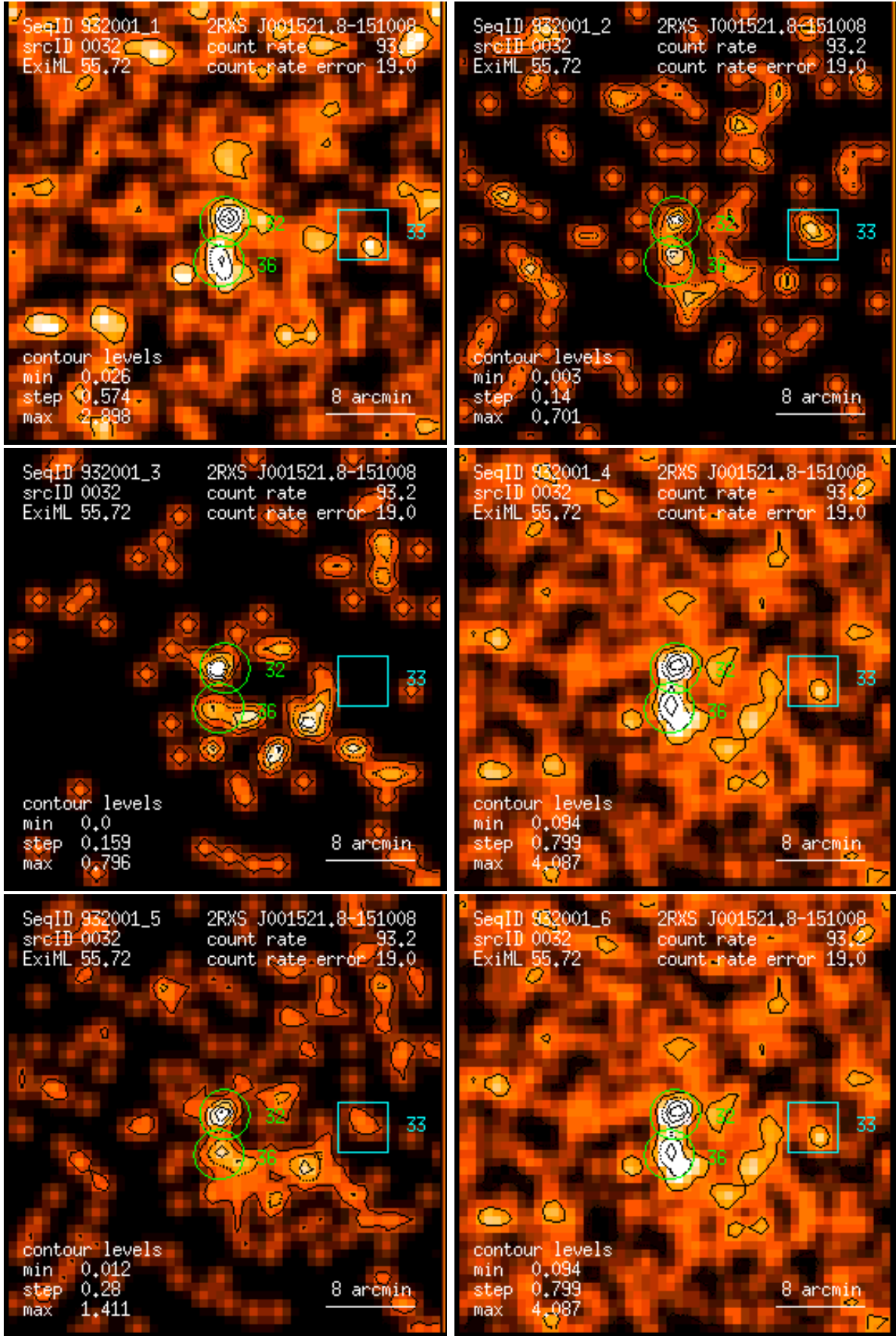
Figure 32: RASS 932001: detection 0032: band rate images, Gaussian filter: (1) PSPC channels 11 – 41, (2) 52 – 90, (3) 91 – 201, (4) 11 – 235, (5) 52 – 201, (6) 11 – 201. Broad band rates in counts/ks. Band rate contour levels in counts/ks/arcmin 2 .
