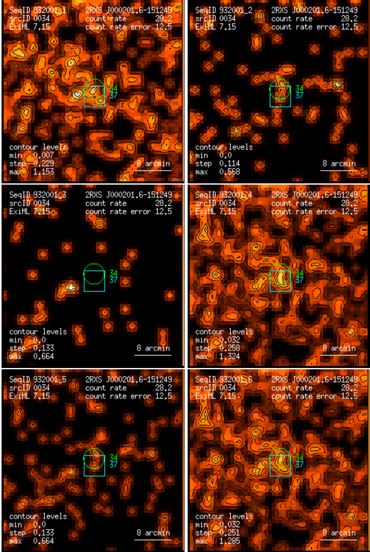
Figure 34: RASS 932001: detection 0034: band rate images, Gaussian filter: (1) PSPC channels 11 – 41, (2) 52 – 90, (3) 91 – 201, (4) 11 – 235, (5) 52 – 201, (6) 11 – 201. Broad band rates in counts/ks. Band rate contour levels in counts/ks/arcmin 2 .
