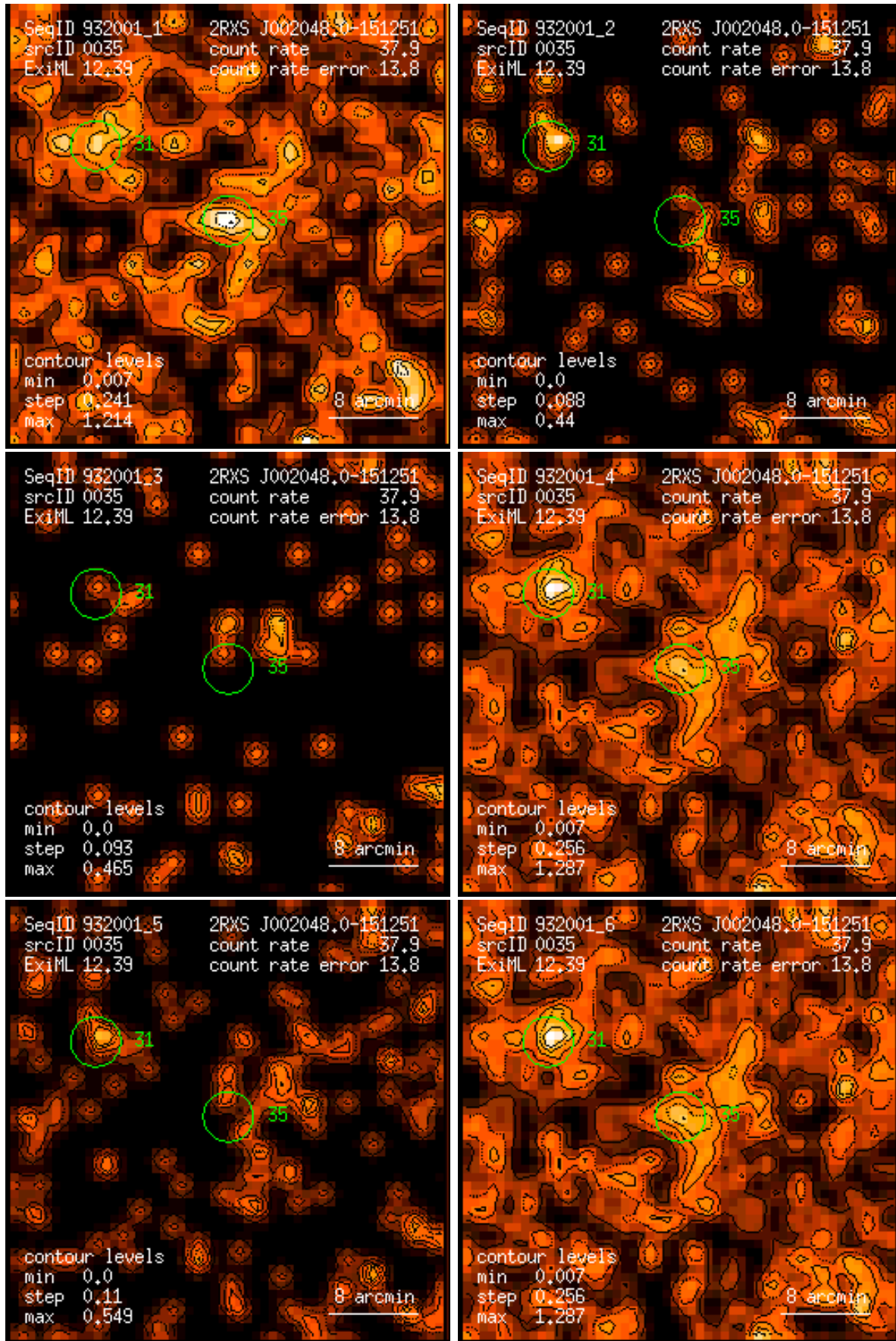
Figure 35: RASS 932001: detection 0035: band rate images, Gaussian filter: (1) PSPC channels 11 – 41, (2) 52 – 90, (3) 91 – 201, (4) 11 – 235, (5) 52 – 201, (6) 11 – 201. Broad band rates in counts/ks. Band rate contour levels in counts/ks/arcmin 2 .
