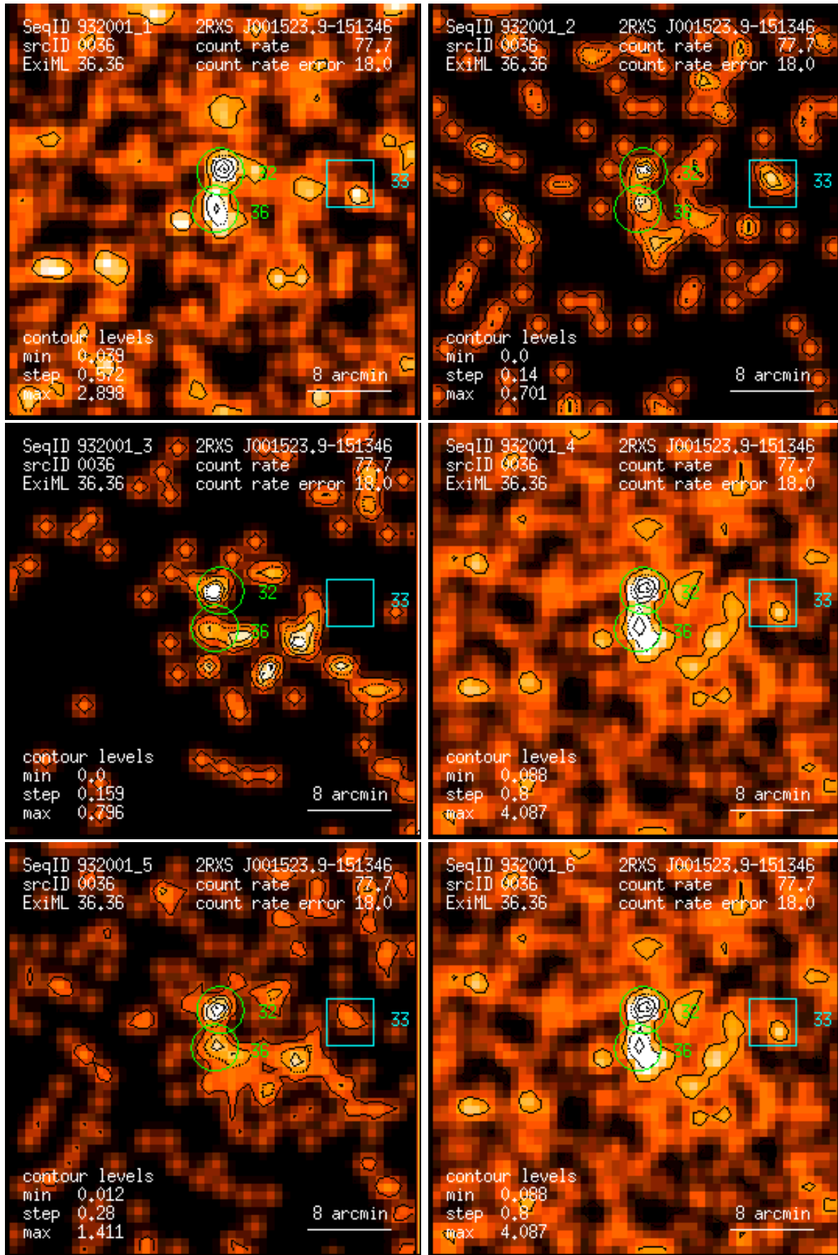
Figure 36: RASS 932001: detection 0036: band rate images, Gaussian filter: (1) PSPC channels 11 – 41, (2) 52 – 90, (3) 91 – 201, (4) 11 – 235, (5) 52 – 201, (6) 11 – 201. Broad band rates in counts/ks. Band rate contour levels in counts/ks/arcmin 2 .
