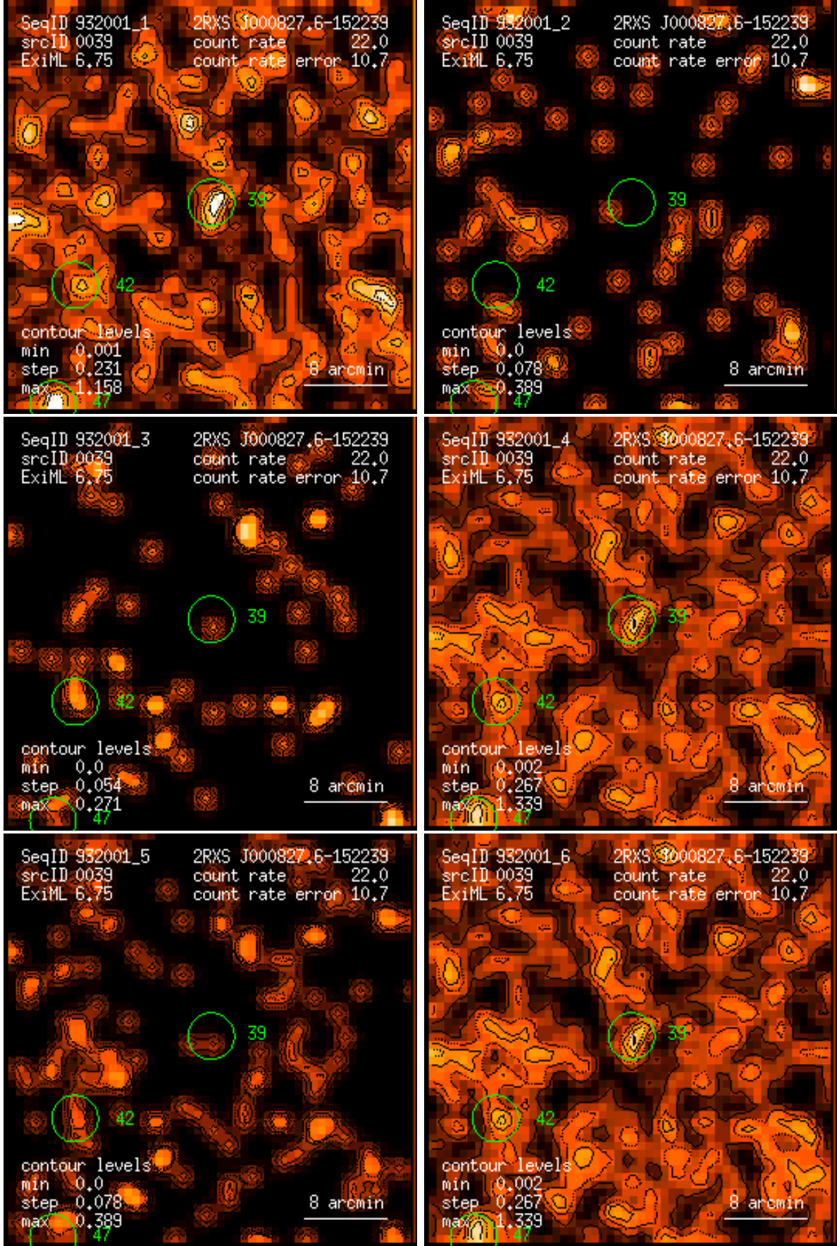
Figure 39: RASS 932001: detection 0039: band rate images, Gaussian filter: (1) PSPC channels 11 – 41, (2) 52 – 90, (3) 91 – 201, (4) 11 – 235, (5) 52 – 201, (6) 11 – 201. Broad band rates in counts/ks. Band rate contour levels in counts/ks/arcmin 2 .
