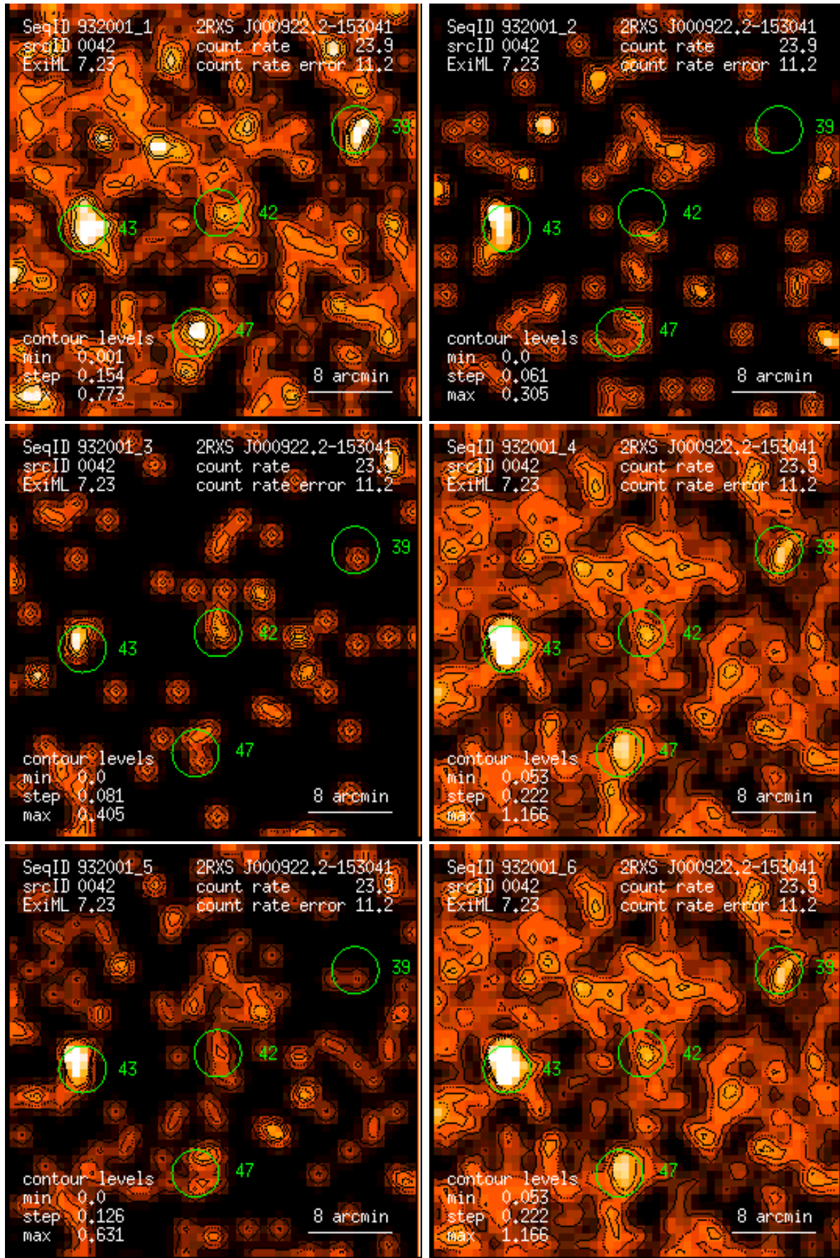
Figure 42: RASS 932001: detection 0042: band rate images, Gaussian filter: (1) PSPC channels 11 – 41, (2) 52 – 90, (3) 91 – 201, (4) 11 – 235, (5) 52 – 201, (6) 11 – 201. Broad band rates in counts/ks. Band rate contour levels in counts/ks/arcmin 2 .
