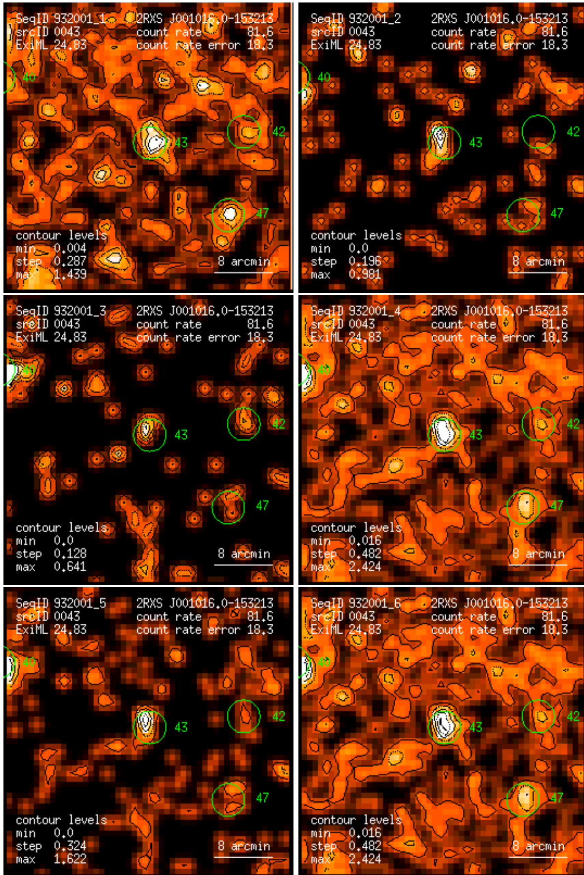
Figure 43: RASS 932001: detection 0043: band rate images, Gaussian filter: (1) PSPC channels 11 – 41, (2) 52 – 90, (3) 91 – 201, (4) 11 – 235, (5) 52 – 201, (6) 11 – 201. Broad band rates in counts/ks. Band rate contour levels in counts/ks/arcmin 2 .
