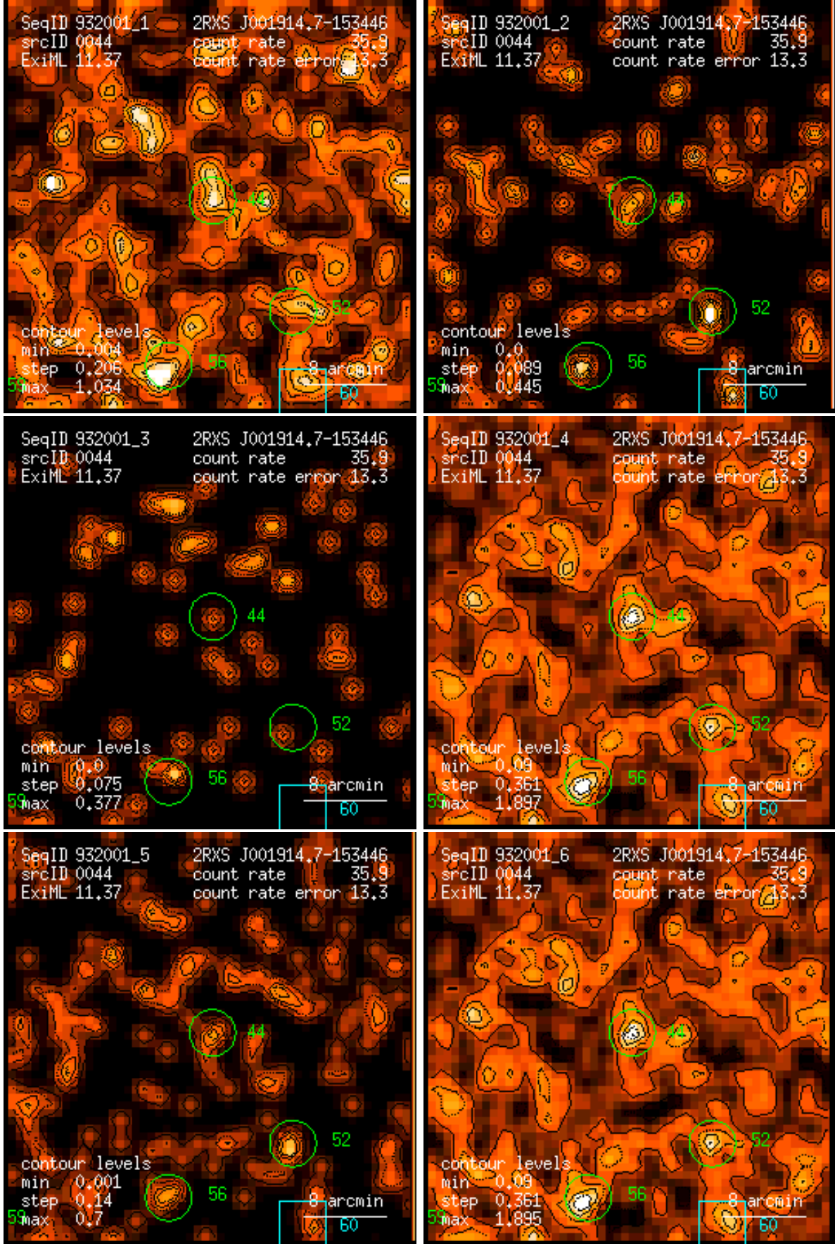
Figure 44: RASS 932001: detection 0044: band rate images, Gaussian filter: (1) PSPC channels 11 – 41, (2) 52 – 90, (3) 91 – 201, (4) 11 – 235, (5) 52 – 201, (6) 11 – 201. Broad band rates in counts/ks. Band rate contour levels in counts/ks/arcmin 2 .
