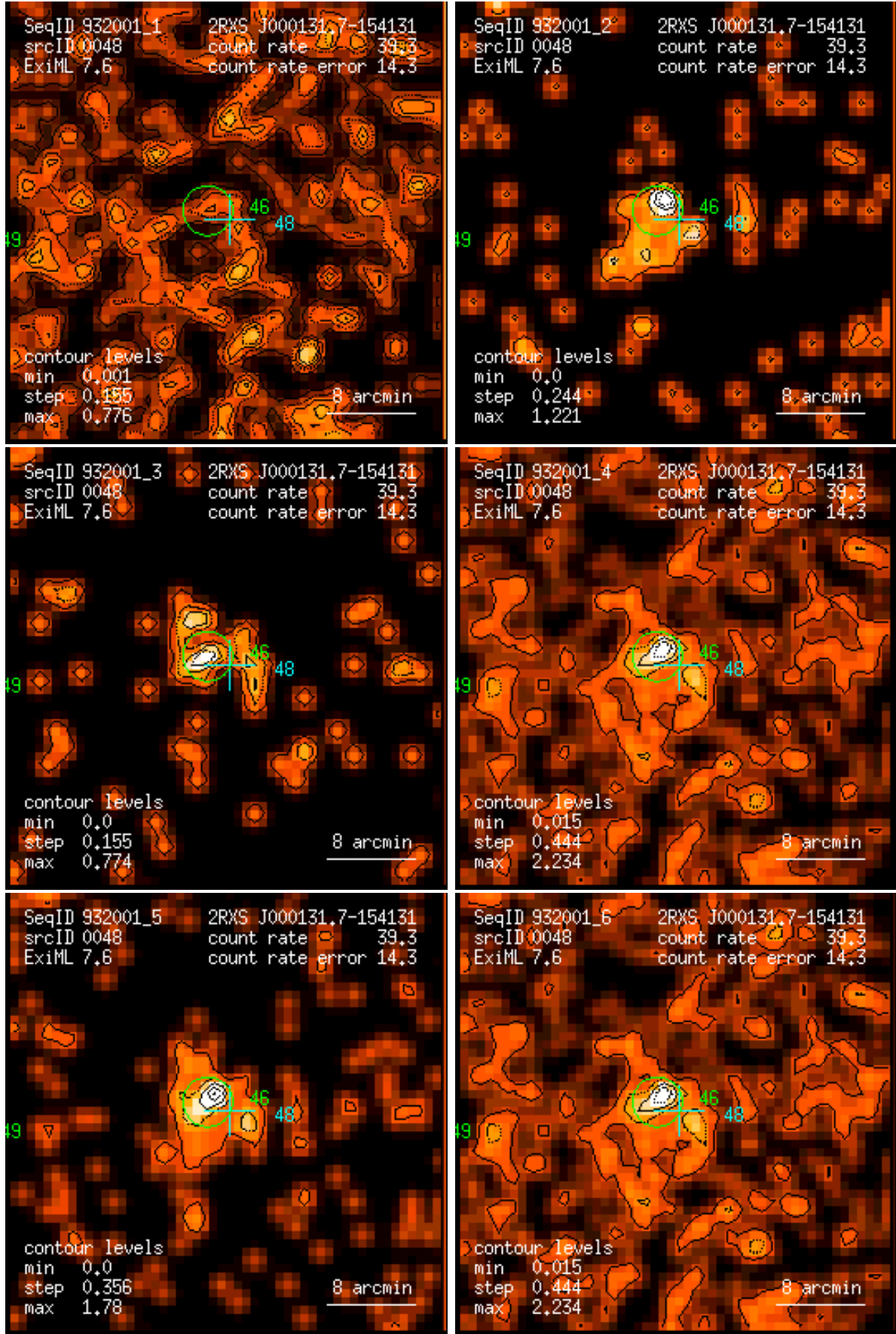
Figure 48: RASS 932001: detection 0048: band rate images, Gaussian filter: (1) PSPC channels 11 – 41, (2) 52 – 90, (3) 91 – 201, (4) 11 – 235, (5) 52 – 201, (6) 11 – 201. Broad band rates in counts/ks. Band rate contour levels in counts/ks/arcmin 2 .
