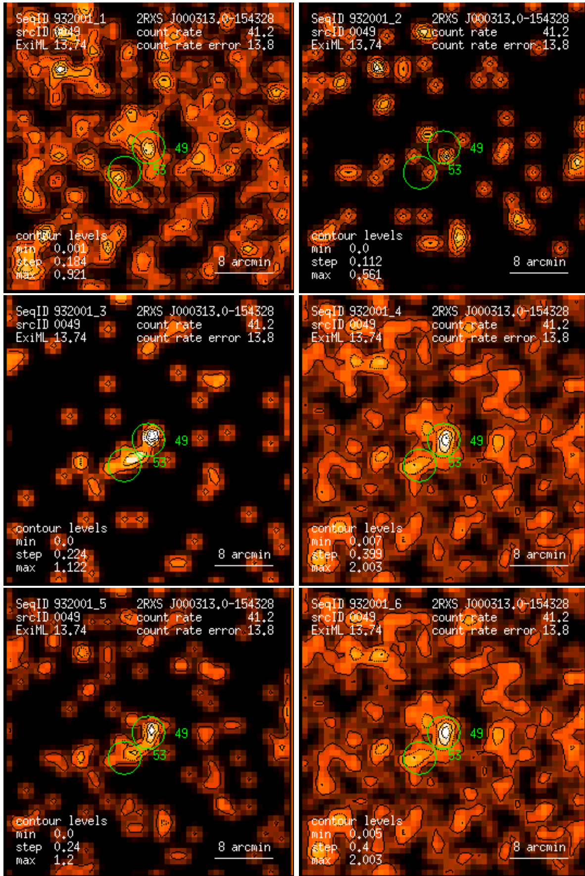
Figure 49: RASS 932001: detection 0049: band rate images, Gaussian filter: (1) PSPC channels 11 – 41, (2) 52 – 90, (3) 91 – 201, (4) 11 – 235, (5) 52 – 201, (6) 11 – 201. Broad band rates in counts/ks. Band rate contour levels in counts/ks/arcmin 2 .
