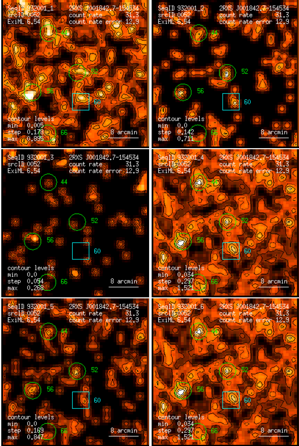
Figure 52: RASS 932001: detection 0052: band rate images, Gaussian filter: (1) PSPC channels 11 – 41, (2) 52 – 90, (3) 91 – 201, (4) 11 – 235, (5) 52 – 201, (6) 11 – 201. Broad band rates in counts/ks. Band rate contour levels in counts/ks/arcmin 2 .
