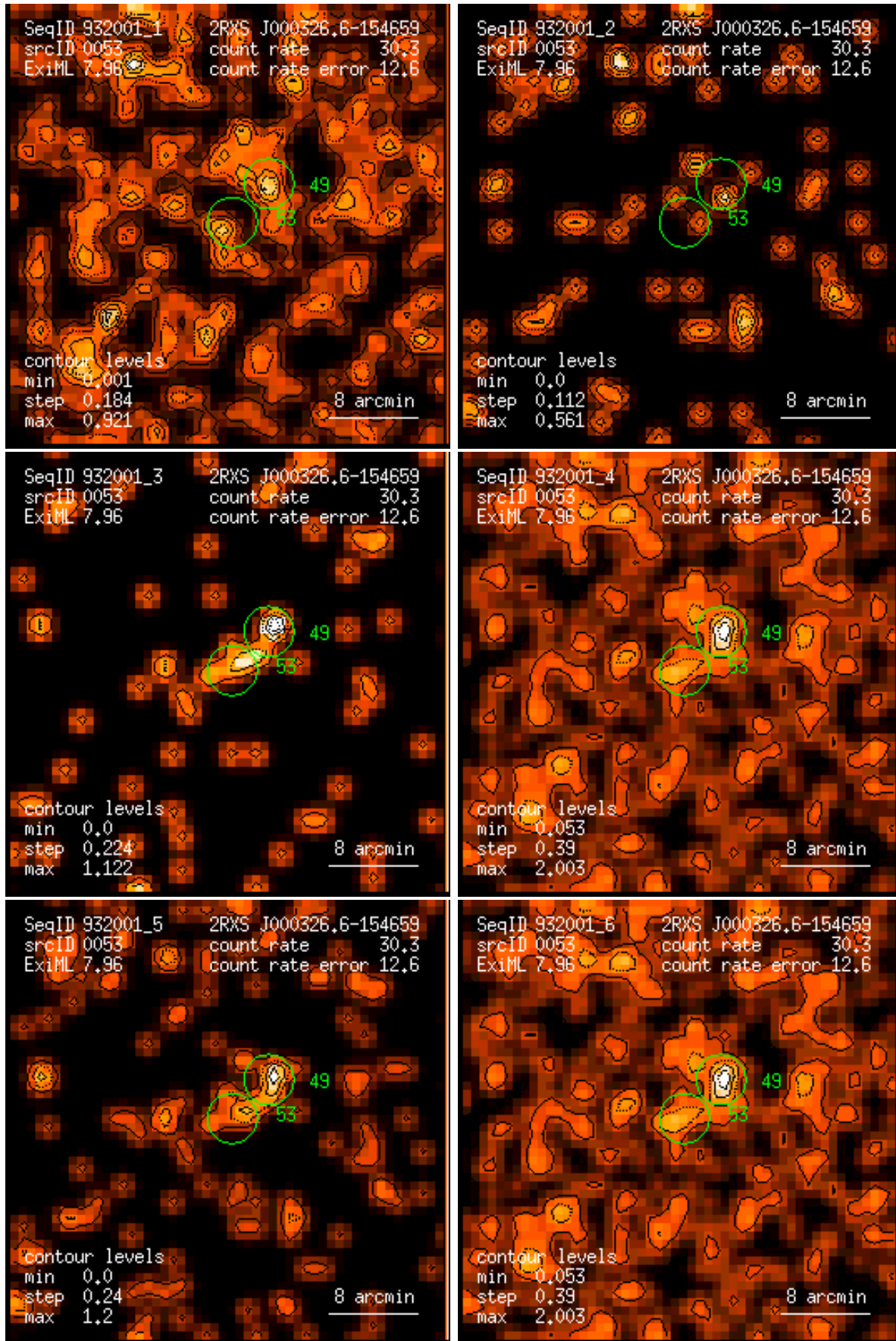
Figure 53: RASS 932001: detection 0053: band rate images, Gaussian filter: (1) PSPC channels 11 – 41, (2) 52 – 90, (3) 91 – 201, (4) 11 – 235, (5) 52 – 201, (6) 11 – 201. Broad band rates in counts/ks. Band rate contour levels in counts/ks/arcmin 2 .
