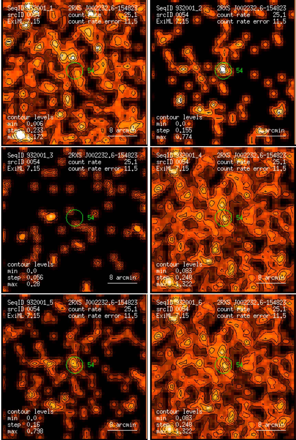
Figure 54: RASS 932001: detection 0054: band rate images, Gaussian filter: (1) PSPC channels 11 – 41, (2) 52 – 90, (3) 91 – 201, (4) 11 – 235, (5) 52 – 201, (6) 11 – 201. Broad band rates in counts/ks. Band rate contour levels in counts/ks/arcmin 2 .
