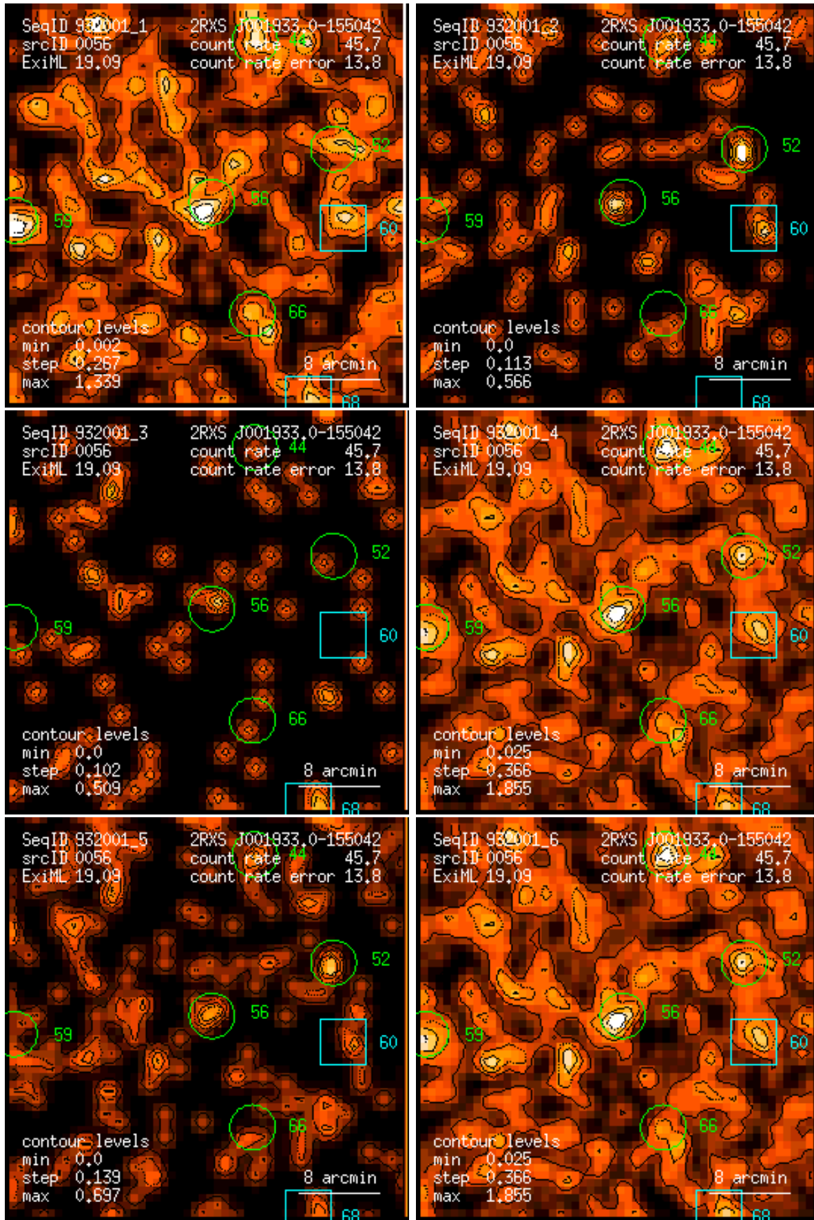
Figure 56: RASS 932001: detection 0056: band rate images, Gaussian filter: (1) PSPC channels 11 – 41, (2) 52 – 90, (3) 91 – 201, (4) 11 – 235, (5) 52 – 201, (6) 11 – 201. Broad band rates in counts/ks. Band rate contour levels in counts/ks/arcmin 2 .
