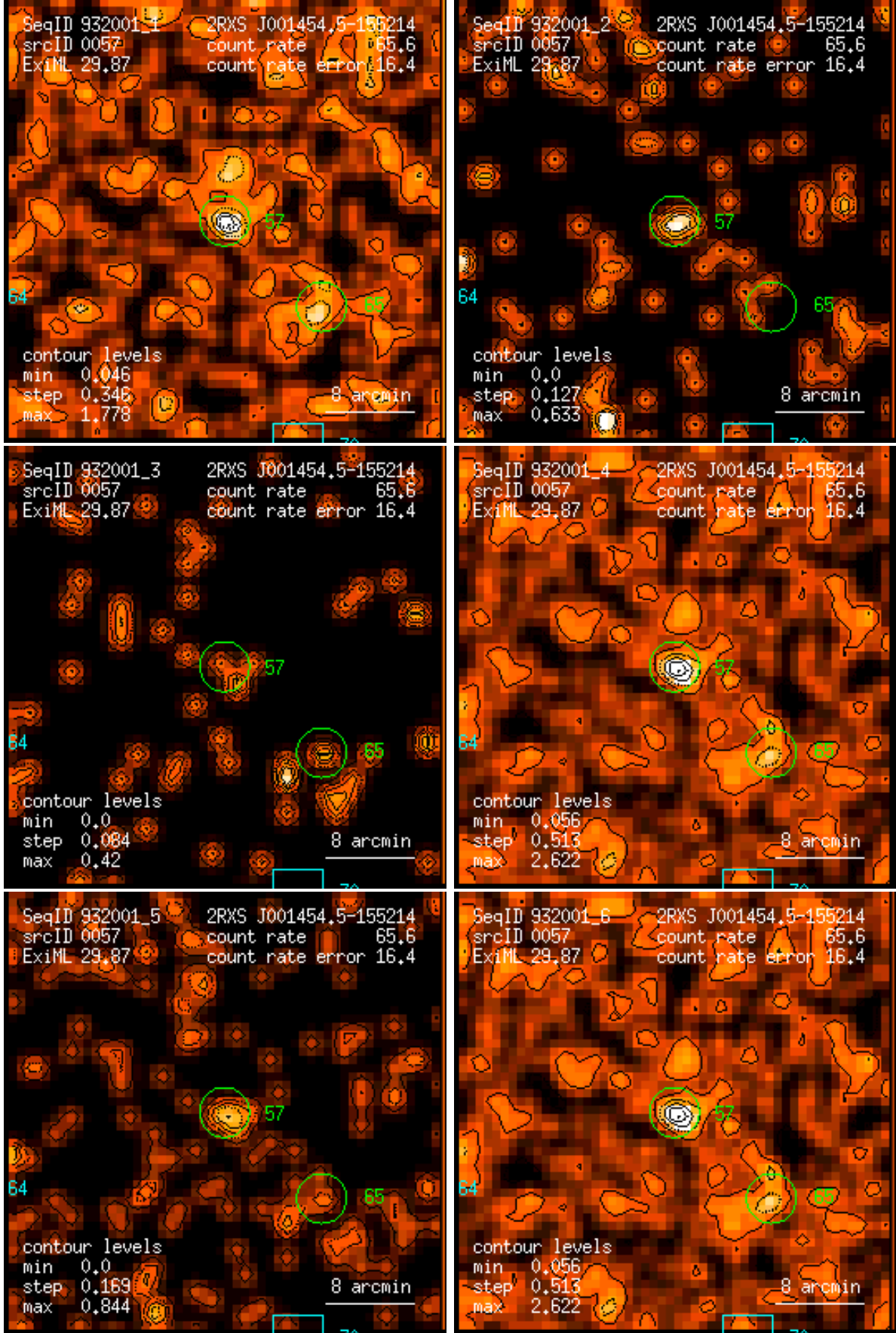
Figure 57: RASS 932001: detection 0057: band rate images, Gaussian filter: (1) PSPC channels 11 – 41, (2) 52 – 90, (3) 91 – 201, (4) 11 – 235, (5) 52 – 201, (6) 11 – 201. Broad band rates in counts/ks. Band rate contour levels in counts/ks/arcmin 2 .
