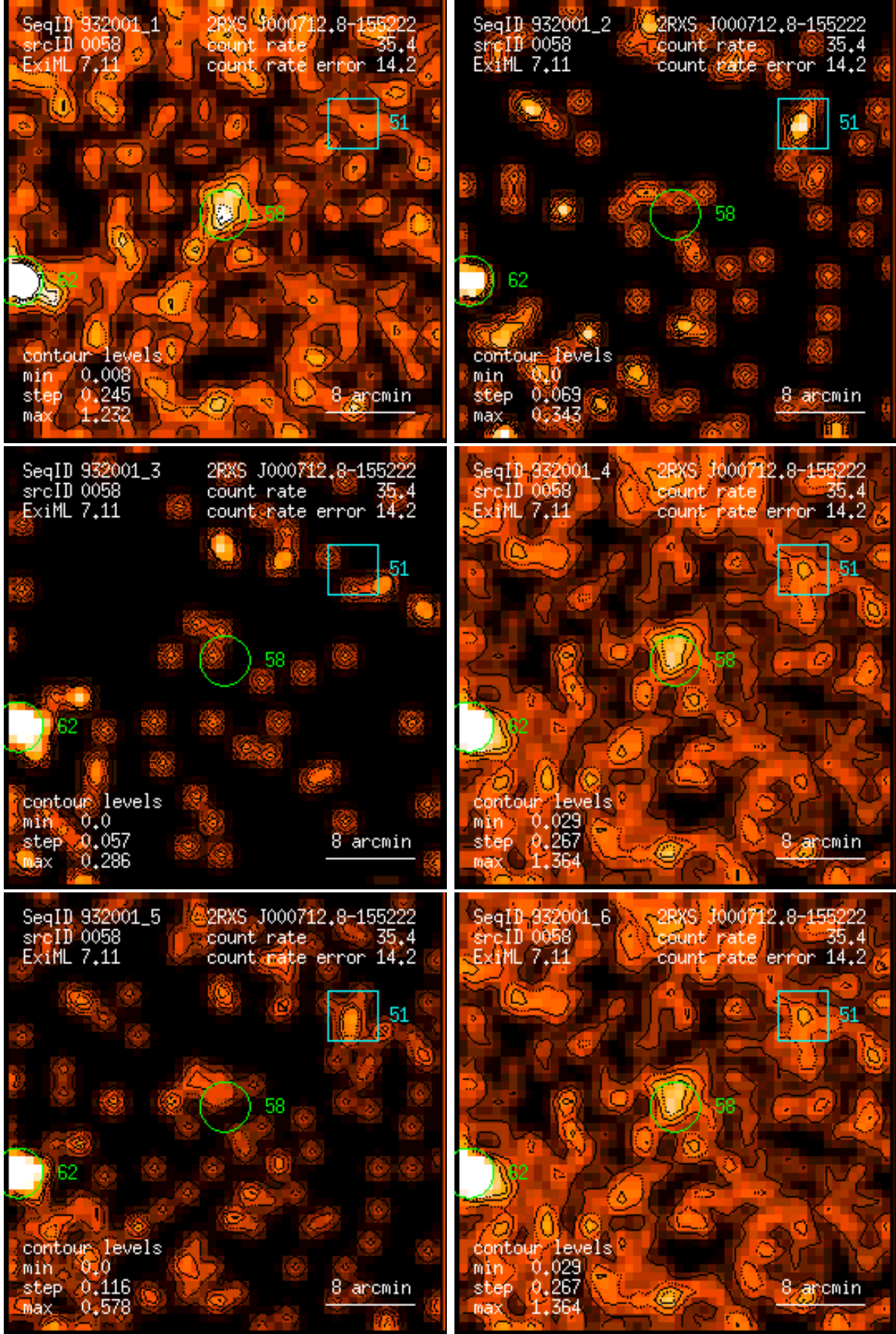
Figure 58: RASS 932001: detection 0058: band rate images, Gaussian filter: (1) PSPC channels 11 – 41, (2) 52 – 90, (3) 91 – 201, (4) 11 – 235, (5) 52 – 201, (6) 11 – 201. Broad band rates in counts/ks. Band rate contour levels in counts/ks/arcmin 2 .
