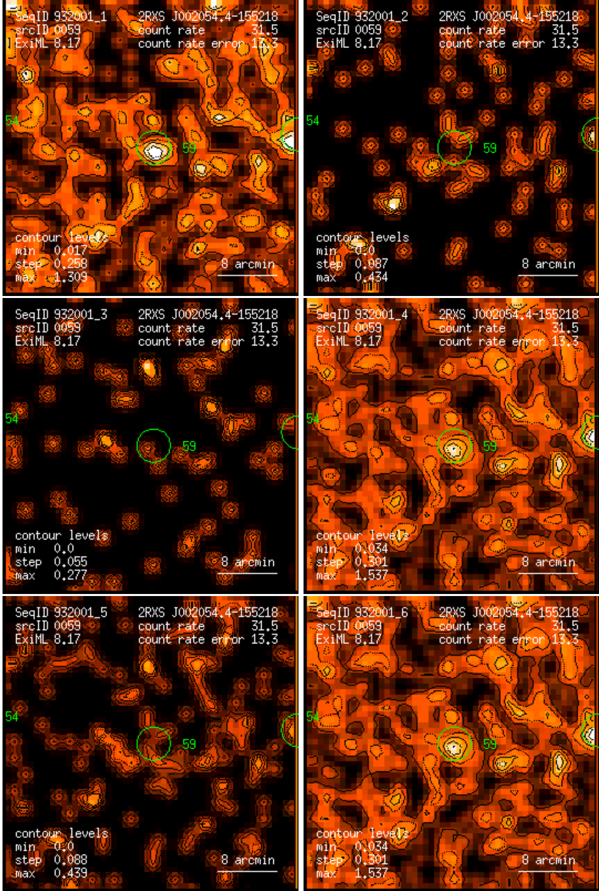
Figure 59: RASS 932001: detection 0059: band rate images, Gaussian filter: (1) PSPC channels 11 – 41, (2) 52 – 90, (3) 91 – 201, (4) 11 – 235, (5) 52 – 201, (6) 11 – 201. Broad band rates in counts/ks. Band rate contour levels in counts/ks/arcmin 2 .
