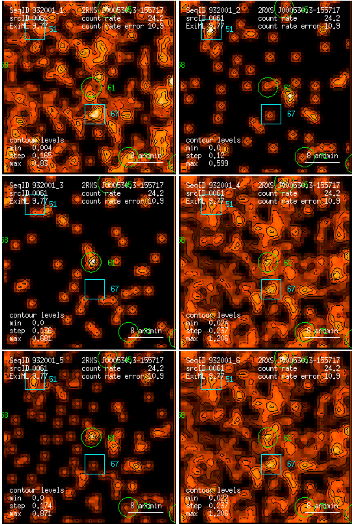
Figure 61: RASS 932001: detection 0061: band rate images, Gaussian filter: (1) PSPC channels 11 – 41, (2) 52 – 90, (3) 91 – 201, (4) 11 – 235, (5) 52 – 201, (6) 11 – 201. Broad band rates in counts/ks. Band rate contour levels in counts/ks/arcmin 2 .
